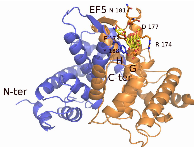
Figure 6. X-ray crystal structure of sorcin in complex with doxorubicin. The chemotherapeutic drug binds close to residues of the EF5 hand, interacting with residues of sorcin G- and H-helices. The two monomers of the sorcin dimer are colored blue and orange. The doxorubicin molecule (colored in yellow) and the residues interacting with it are represented as sticks.
