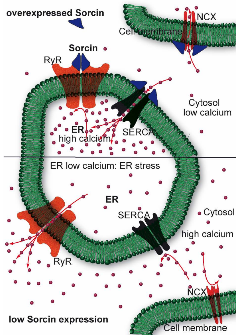
Figure 4. Sorcin inhibits Ryanodine Receptors (RyRs) and activates sarco/endoplasmic reticulum Ca 2+ -ATPase (SERCA) and Na + /Ca 2+ exchanger (NCX), thereby increasing Ca 2+ load of the endoplasmic reticulum (ER) and decreasing ER stress (top). When sorcin expression is low, ER Ca 2+ load is decreased, thereby increasing ER stress (bottom).
