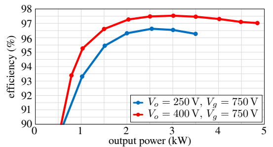
Fig. 13: Efficiency of the topology.
