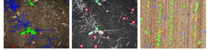
Fig. 4. Example results obtained by our plant classification systems. Left: UGV-based semantic segmentation into crop, weed, grass-weed. Middle: stem detection providing accurate location of crops and weeds. Right: UAV-based semantic segmentation.
