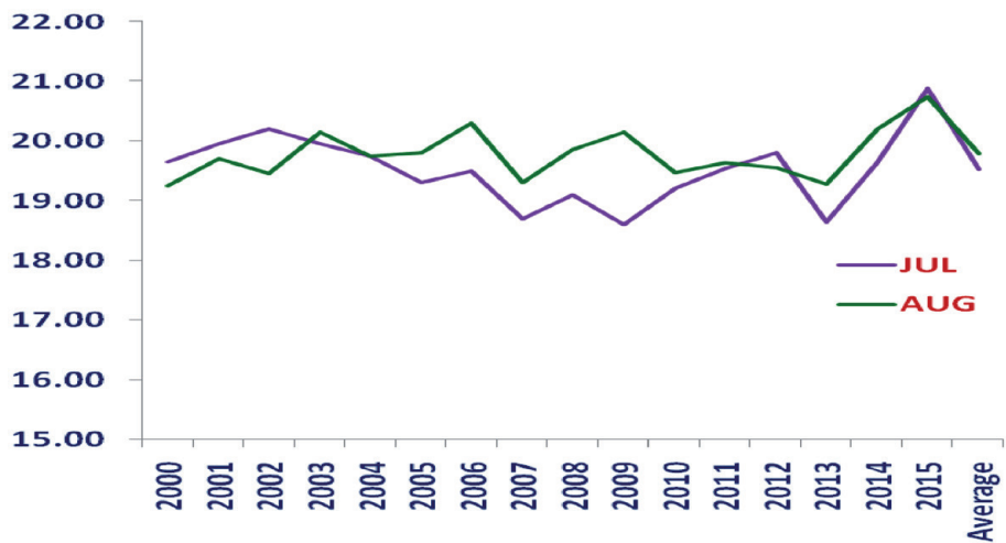
Figure 6. Mean Weather data at Gudalur Location.
