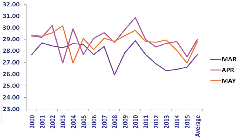
Figure 5. Mean Weather data at Coimbatore Location.
