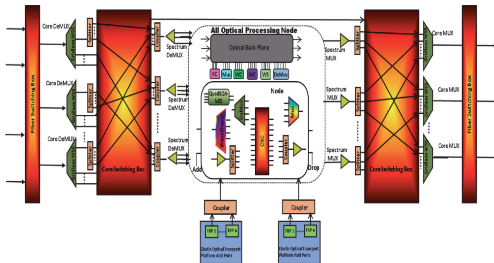
Figure 13. Spatially and spectrally resolved optical switching fabric.
