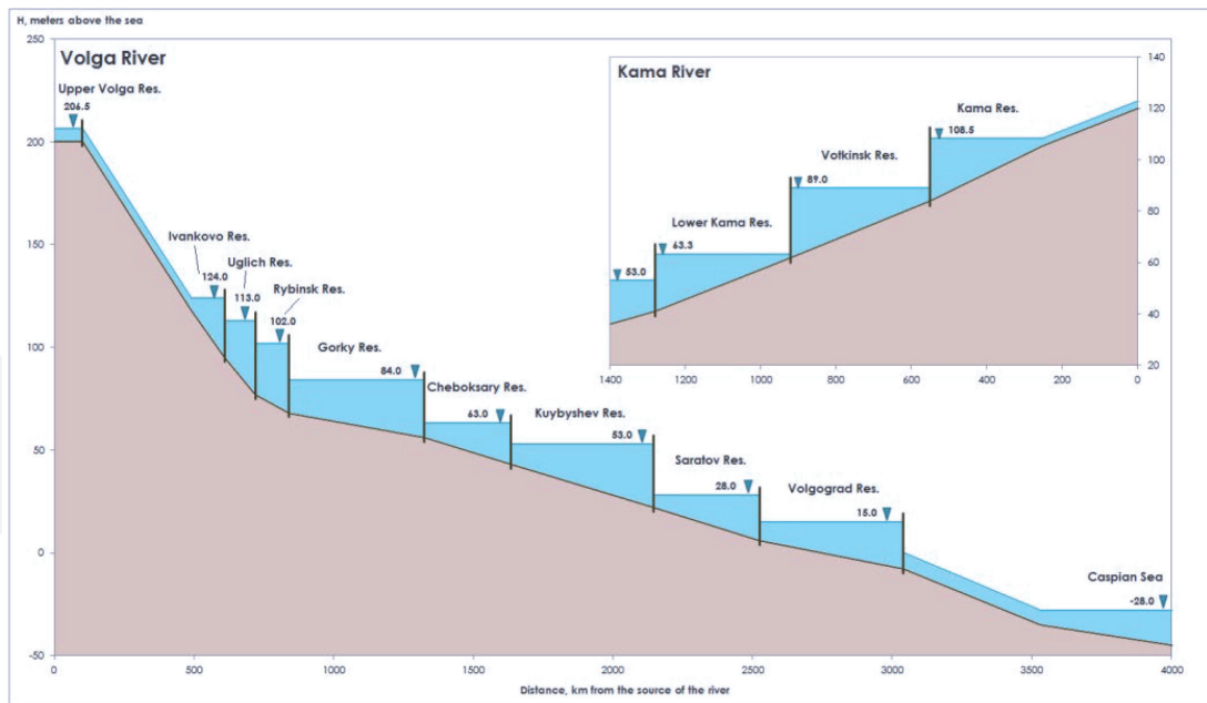
Figure 4. VKC water surface profiles (based on materials [1, 5]).
