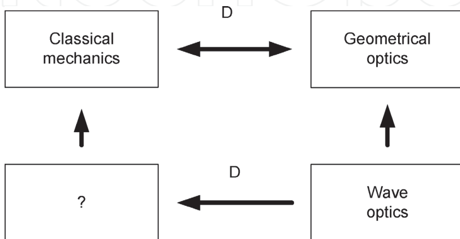
Figure 1. Guessing Schrödinger's equation.
