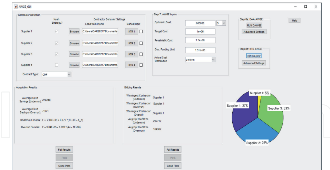
Figure 14. Matlab GUI for system acquisition strategy development and optimization.
