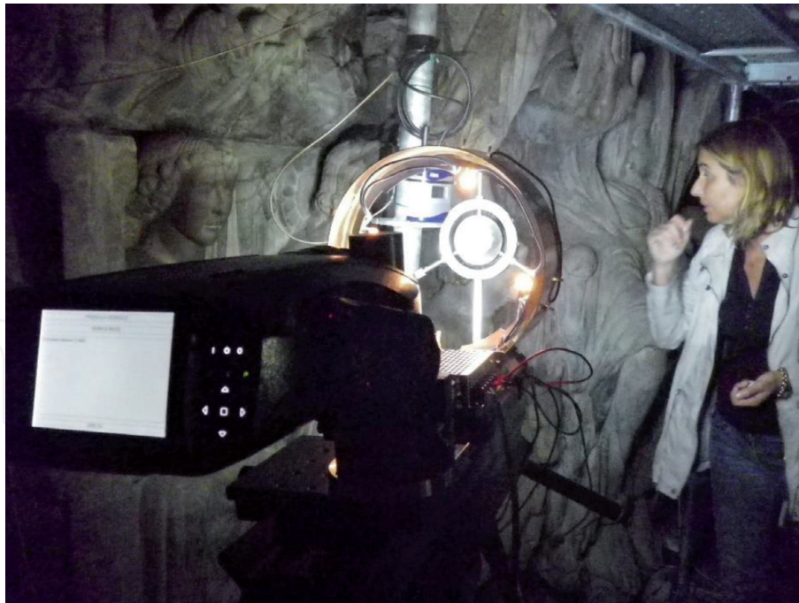
Figure 2. Spectroradiometer with standard white at Pórtico de la Gloria.
