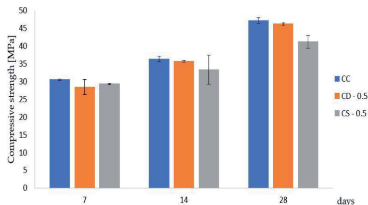
Figure 4. Compressive strength results of concrete samples [29].
