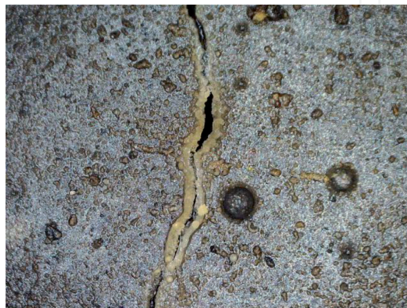
Figure 5. Concrete sample with self-healing process activated [115].
