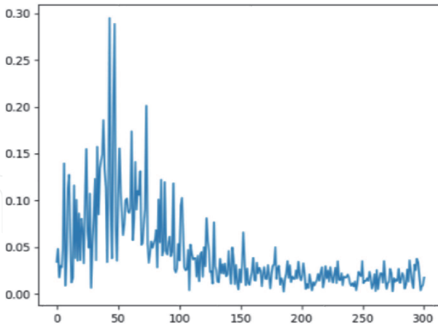
Figure 12. FFT plot with No load on the motor.
