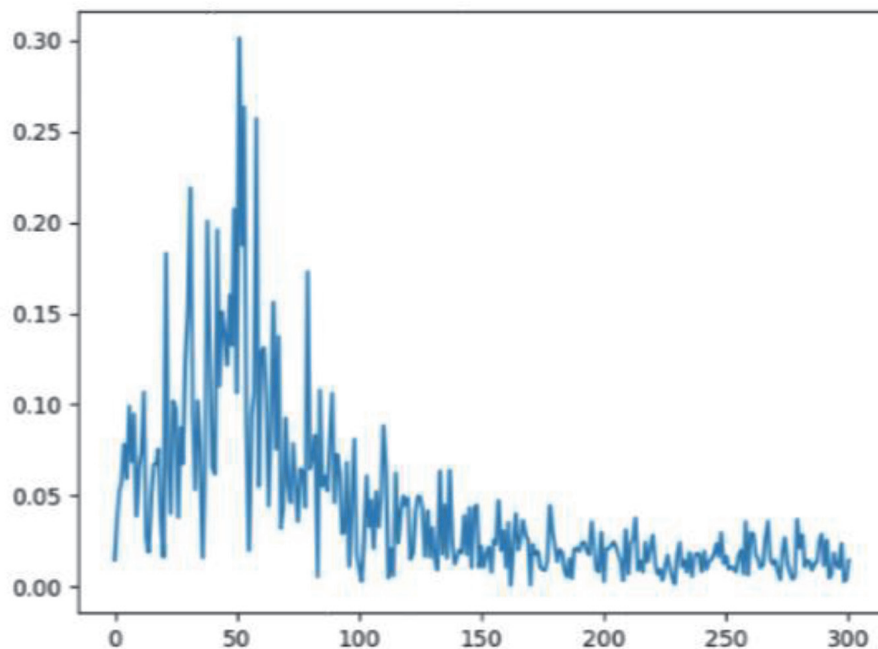
Figure 13. FFT plot with imbalance load on the motor.
