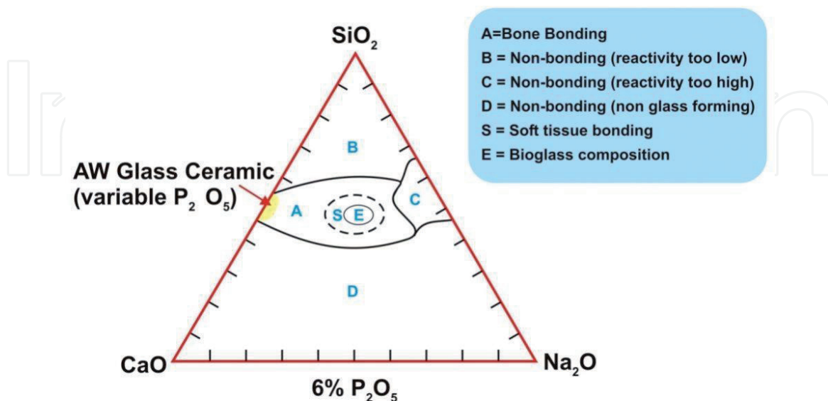
Figure 2. Compositional dependence (wt%) of bone bonding and soft tissue bonding of bioactive glass and glass-ceramics. The compositions within region a have a constant 6% \text{P}_2\text{O}_5 apart from AW glass ceramic which consists of concentration of \text{P}_2\text{O}_5 greater than 6%. Regions S and E both have the ability to interact with and bond to soft tissue and within region E specifically lies the novel bioglass® composition reprinted with permission from [15].
