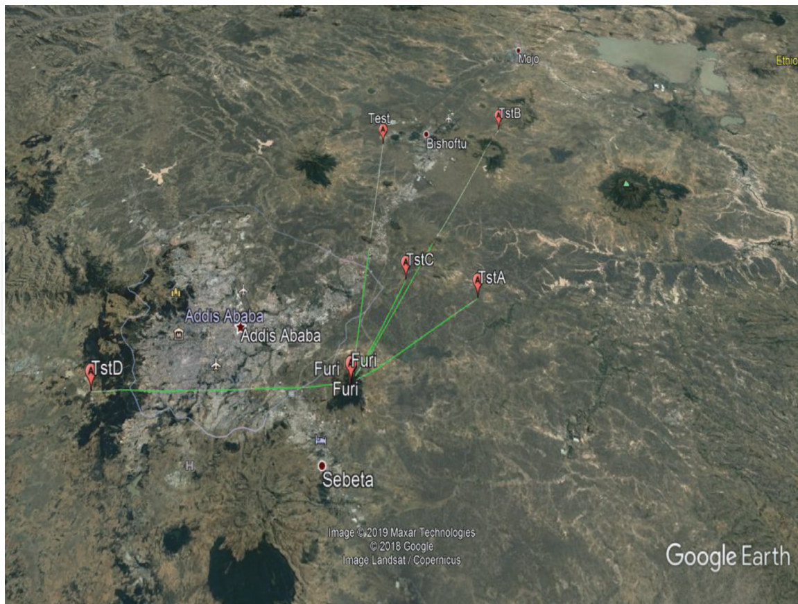
Figure 1. Test points for pathloss analysis (adapted from Google Earth).
