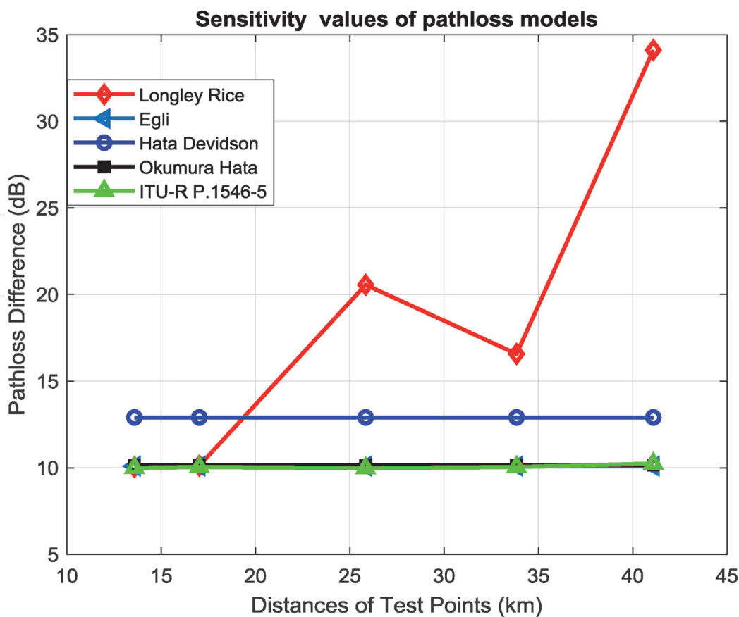
Figure 3. Variations of Pathlosses for VHF and UHF.
