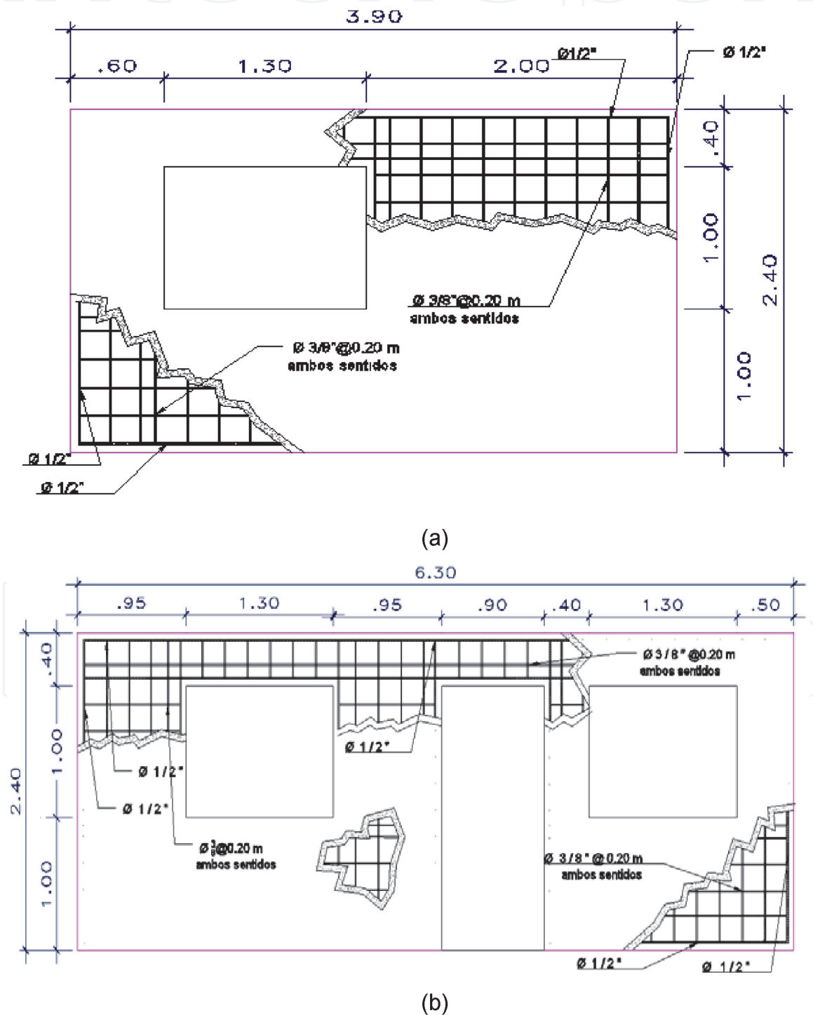
Figure 9. (a) Structure of a side piece with window of the VUF 01. (b) Structure of a front part of the VUF 01.
