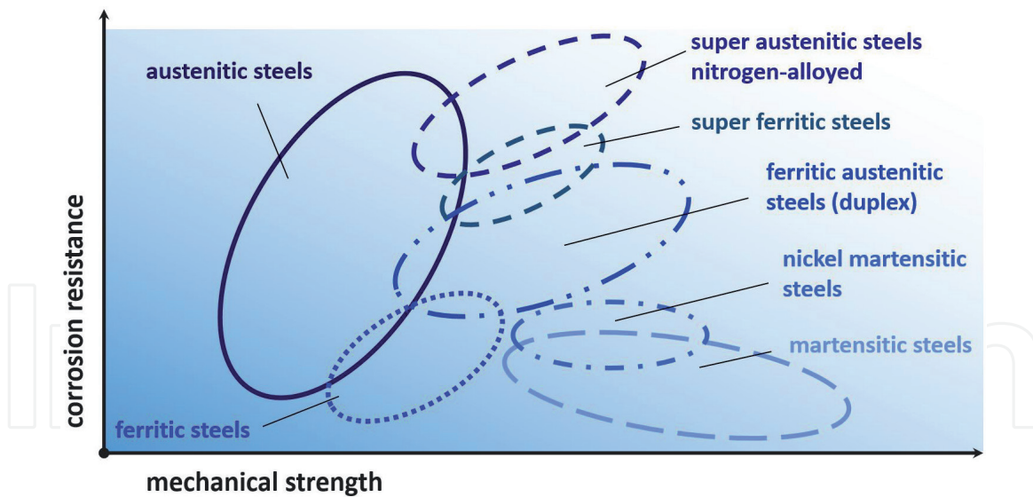
Figure 1. Schematic overview of the relation between corrosion resistance and mechanical strength for the different types of stainless steels [12].
