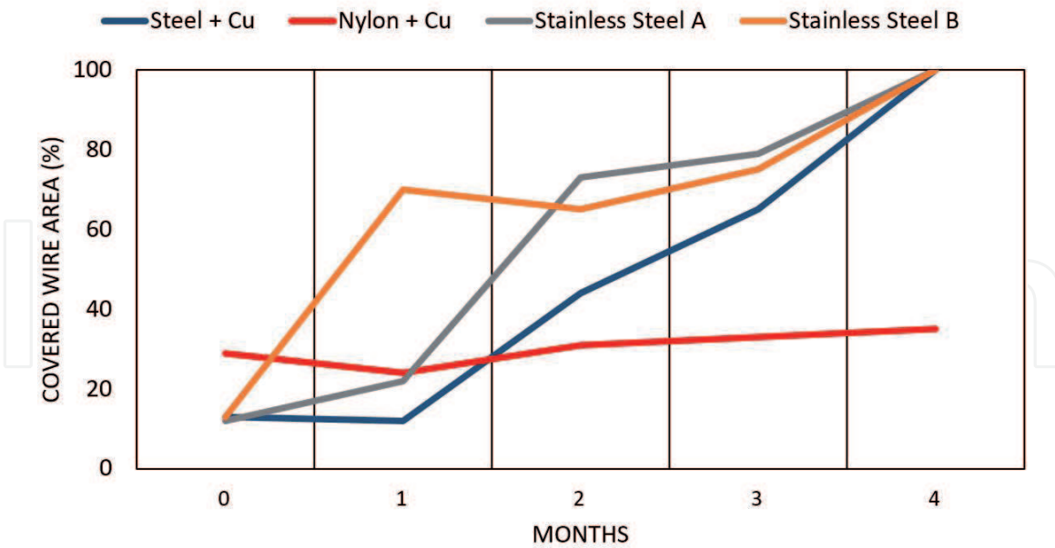
Figure 4. Proportion of the covered area after long-term exposition in seawater (4 months).
