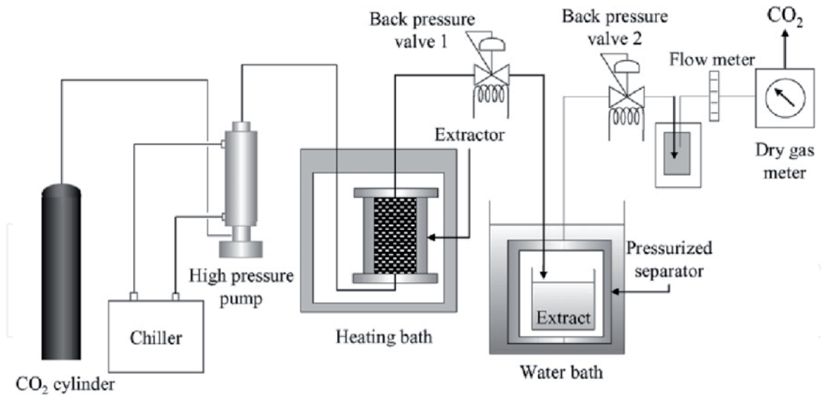
Figure 6. Schematic diagram of supercritical fluid extraction (SFE) set-up [76].
