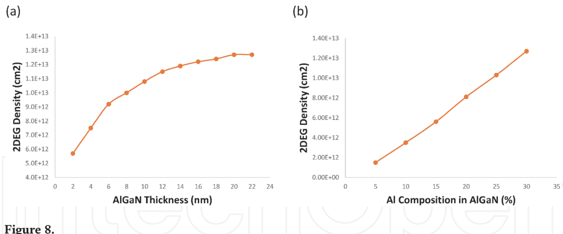
Figure 8. 2DEG carrier concentration of AlGaN/AlN/GaN heterostructure for (a) different AlGaN thickness, (b) different Al composition in AlGaN layer (reprinted with permission from Ref. [12]).
