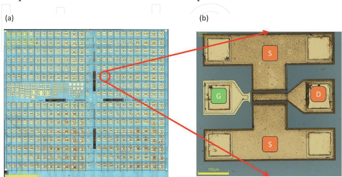
Figure 15. (a) GaN HEMT fabricated wafer (b) 100\text{ nm} \times 200 GaN HEMT device (reprinted with permission from Ref. [56]).
