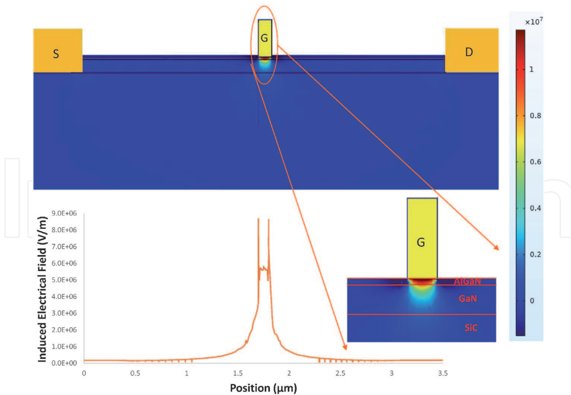
Figure 12. Electrical field enhancement for 0.4 THz incident radiation on GaN HEMT device using a finite element method-based electromagnetic solver (COMSOL).
