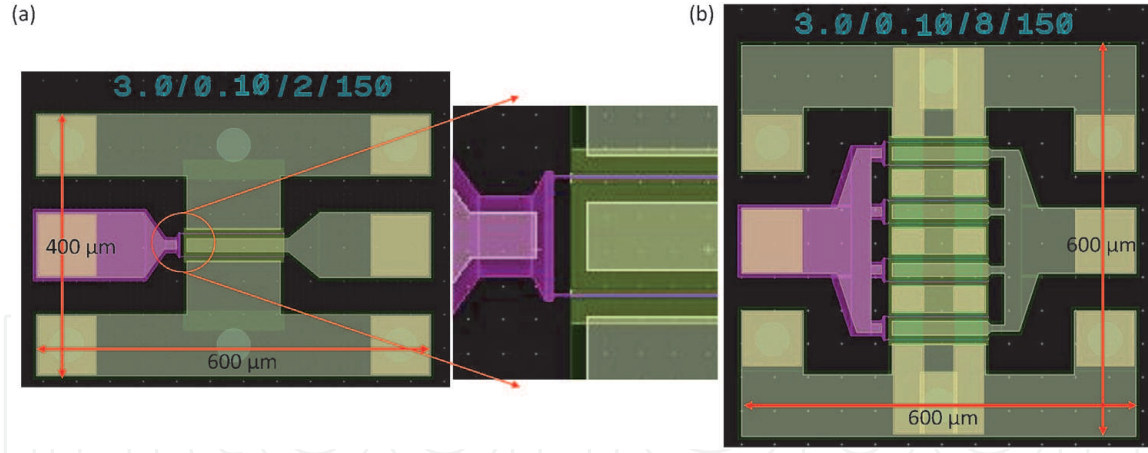
Figure 2. Typical configurations of GaN HEMT (a) 2 gate fingers with 150 micron gate width ( 2 \times 150 ) (zoom image for gate fingers visualization and (b) 8 gate fingers with 150 micron gate width ( 8 \times 150 ). Representation 3.0/0.10/8/150 indicates source to drain distance 3.0 \mu\text{m} , 0.1 \mu\text{m} (100 nm) gate length, 8 fingers device with 150 \mu\text{m} gate width.
