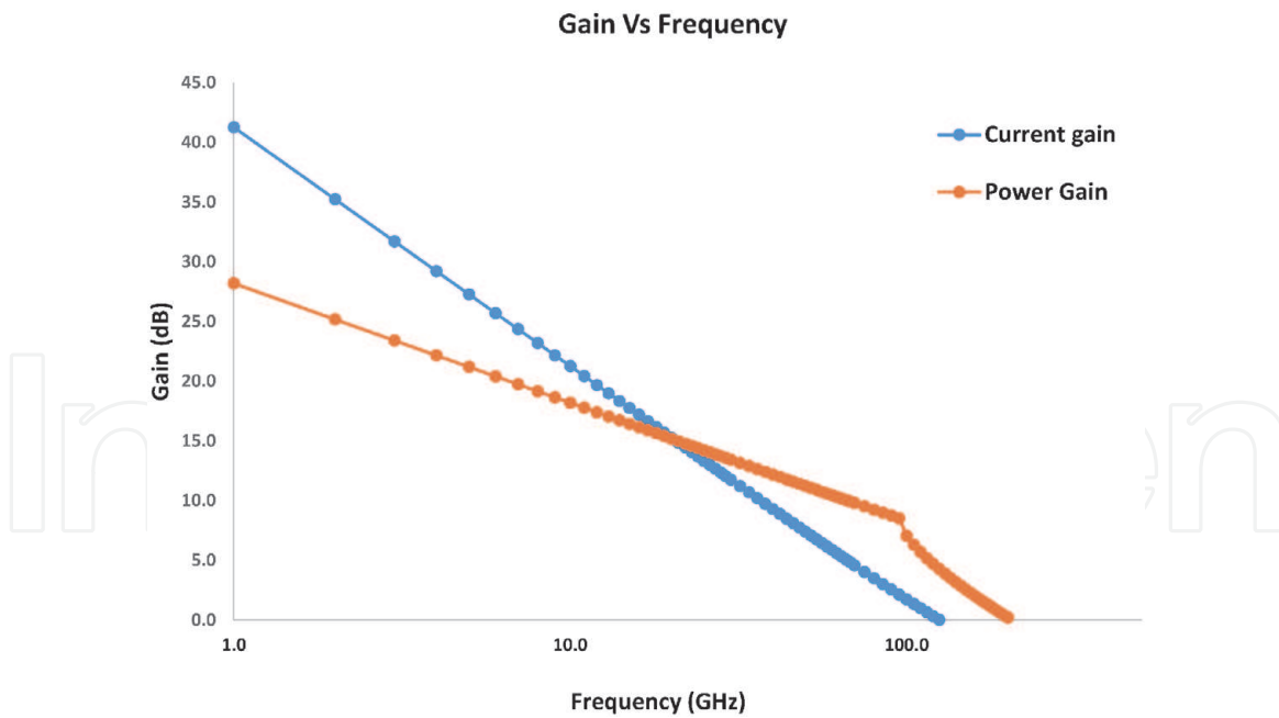
Figure 5. Current gain and power gain of the simulated device (reprinted with permission from Ref. [11]).
