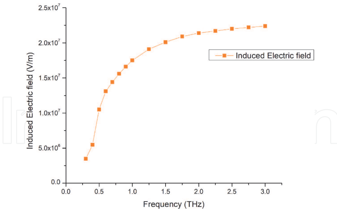
Figure 13. Induced electrical field due to terahertz radiation illumination on GaN HEMT device using a finite element method-based electromagnetic solver (COMSOL).
