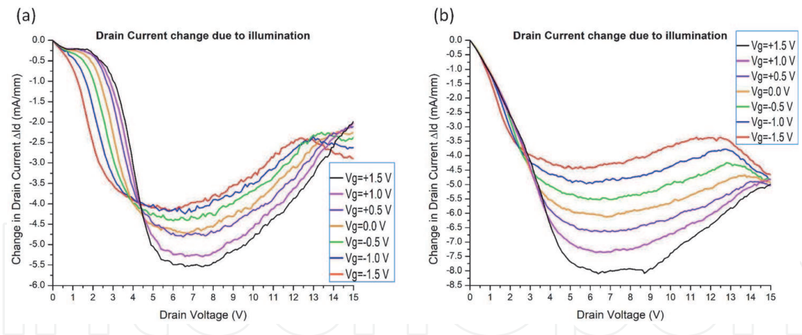
Figure 21. Change in drain current due to 45° AOI and 30° second illumination with SWIRLED at temperature (a) 200 K and (b) 100 K (reprinted with permission from Ref. [56]).
