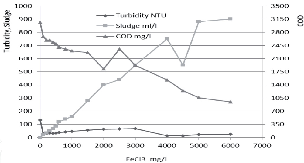
Figure 9. Study of the mixture: \text{FeCl}_3 + ASTRAL flocculant (200 mg/l) variable \text{FeCl}_3 . COD = 3100 mg/l, pH = 6.5.
