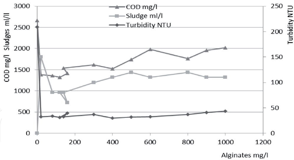
Figure 17. Study of the mixture FeCl_3 (2500 mg/l) + alginate.
