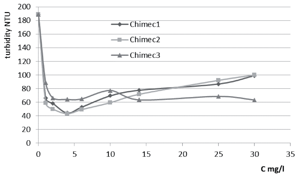
Figure 17. Study of the mixture FeCl_3 (2500 mg/l) + alginate.
