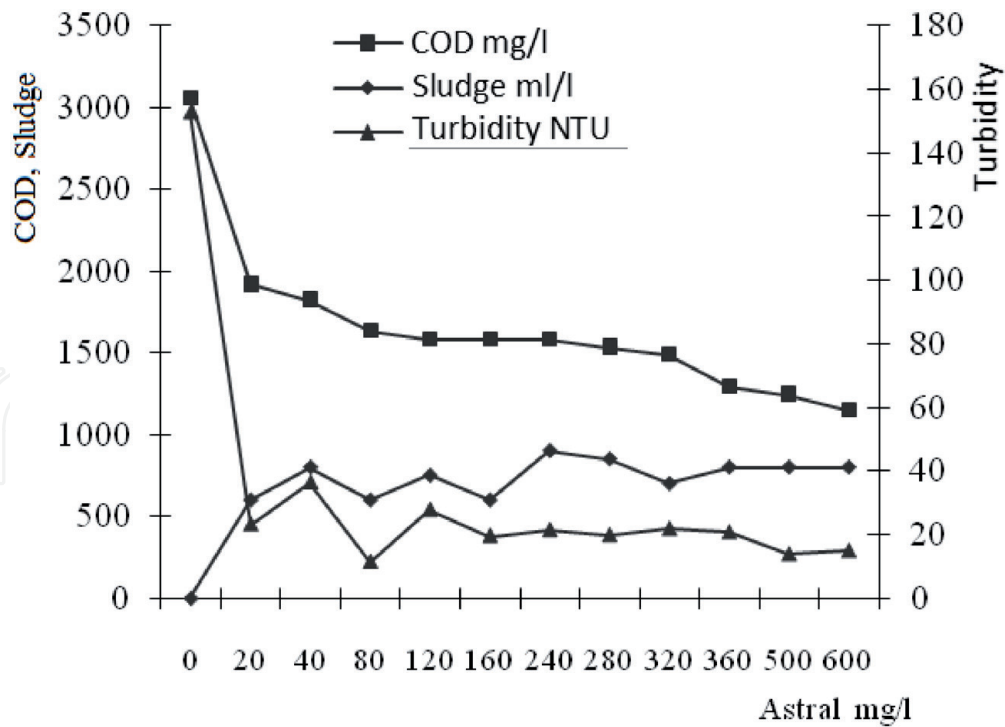
Figure 8. Study of the mixture: \text{FeCl}_3 (2500 mg/l \text{FeCl}_3 ) + Astral flocculant variable flocculant COD = 3056 mg/l, pH = 6.5.
