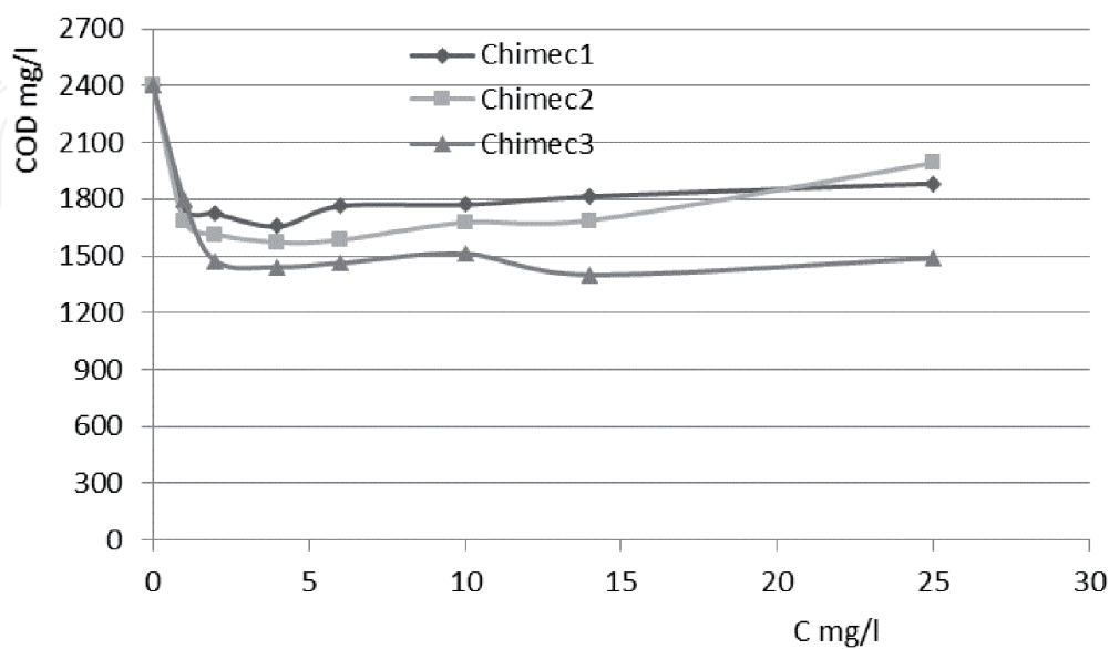
Figure 18. Variation of turbidity (a) and COD (b) during coagulation flocculation by flocculants supplied by an Italian company.
