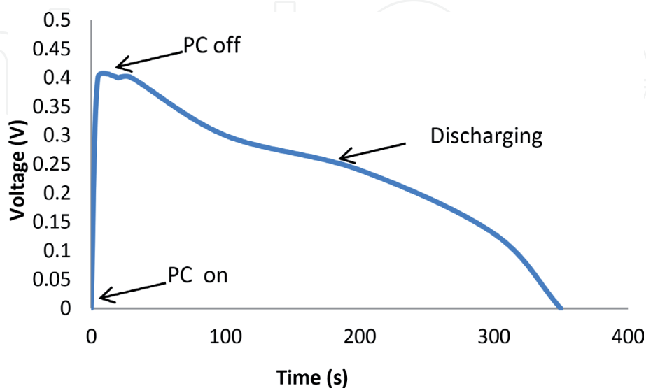
Figure 1. Charging-discharging curve of supercapacitor.
