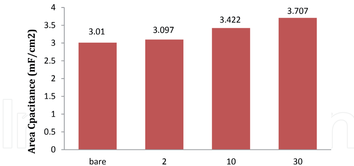
Figure 3. Areal capacitance of CNTs fibers electrodes with different MnO 2 coating.
