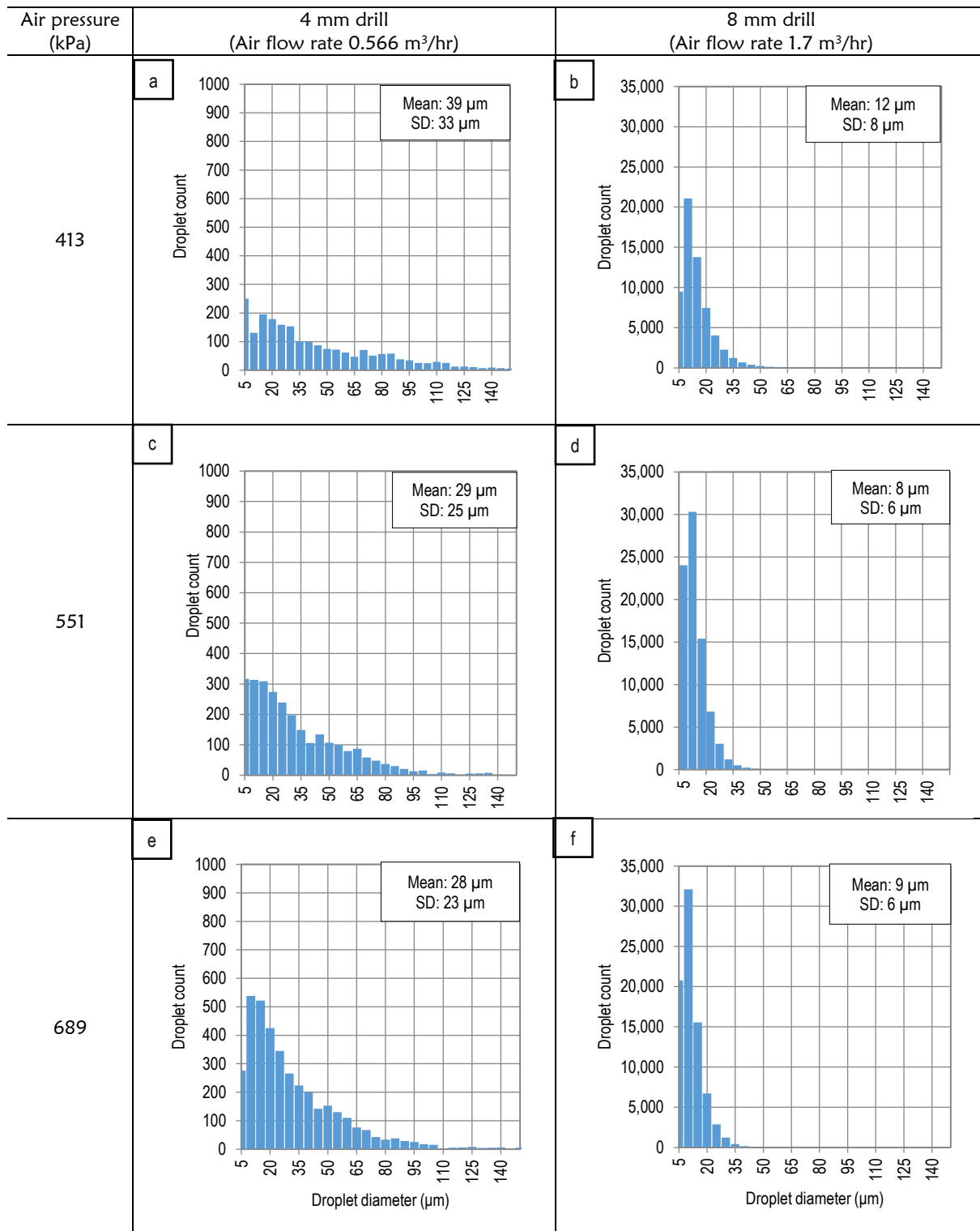
Figure 6. Airborne drop size distribution. Mean and standard deviation of lubricant A's microdroplets at different air pressures.
