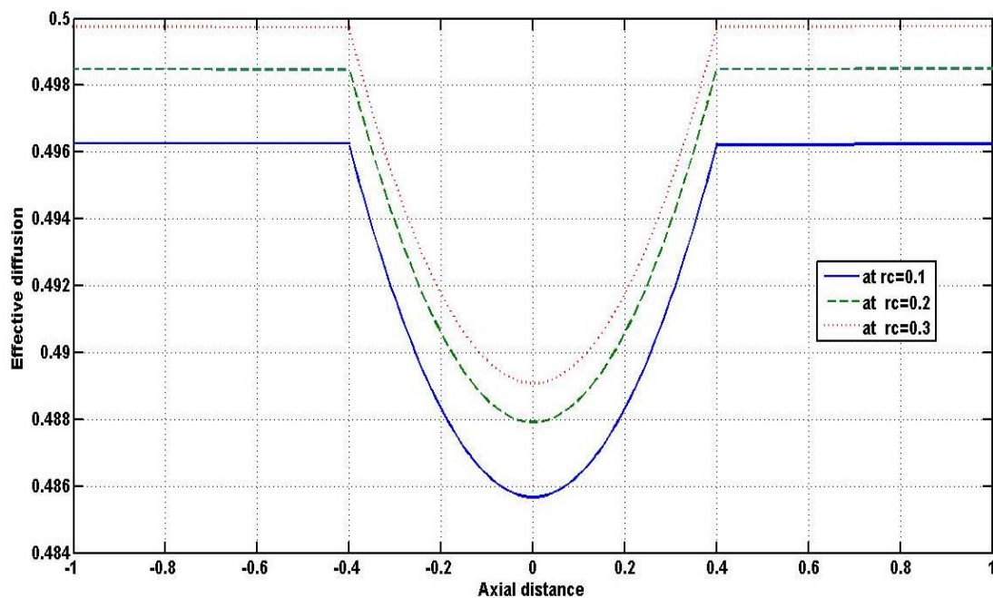
Figure 10. Variation of effective diffusion with axial distance for different rheological parameter r_c
