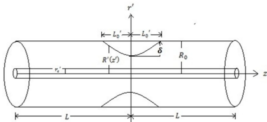
Figure 1. The transport of nanoparticles in a stenosed microvessel
