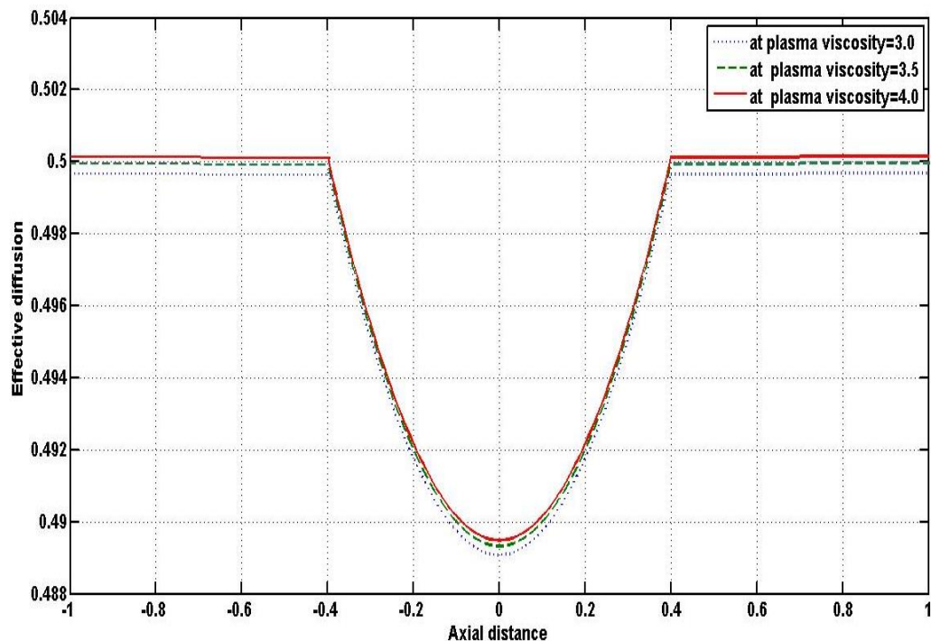
Figure 9. Variation of effective diffusion with axial distance for different plasma viscosity \eta_1
