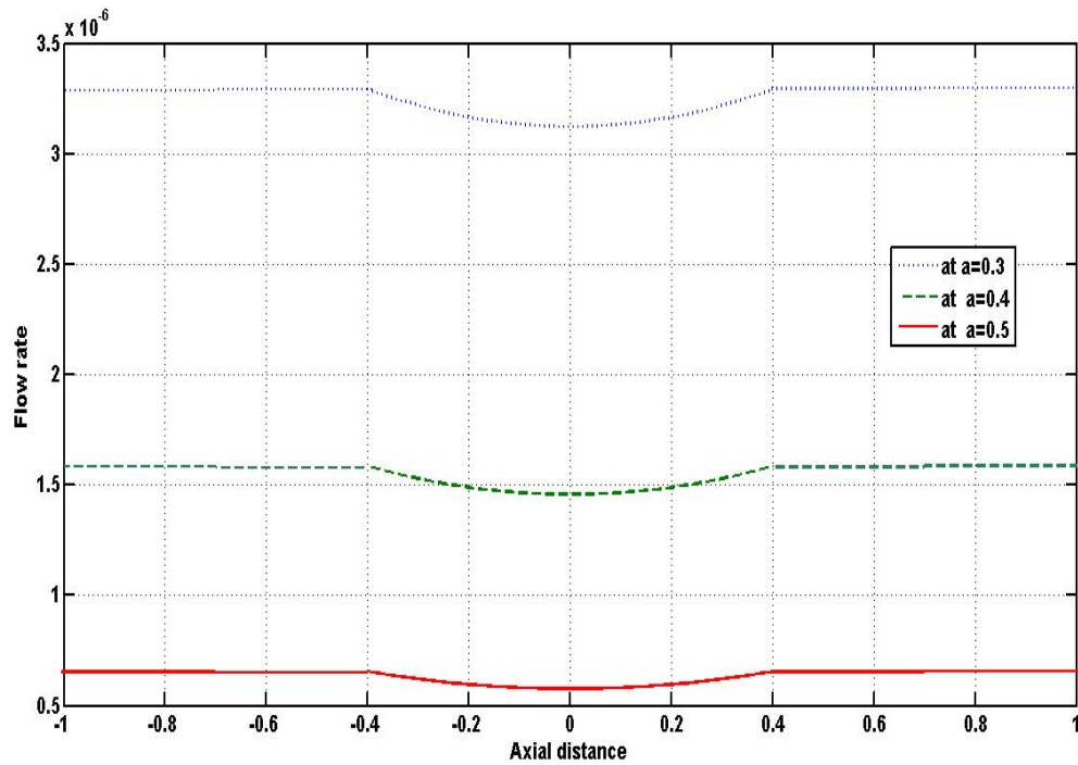
Figure 5. Variation of flow rate with axial distance for different stenosis height a
