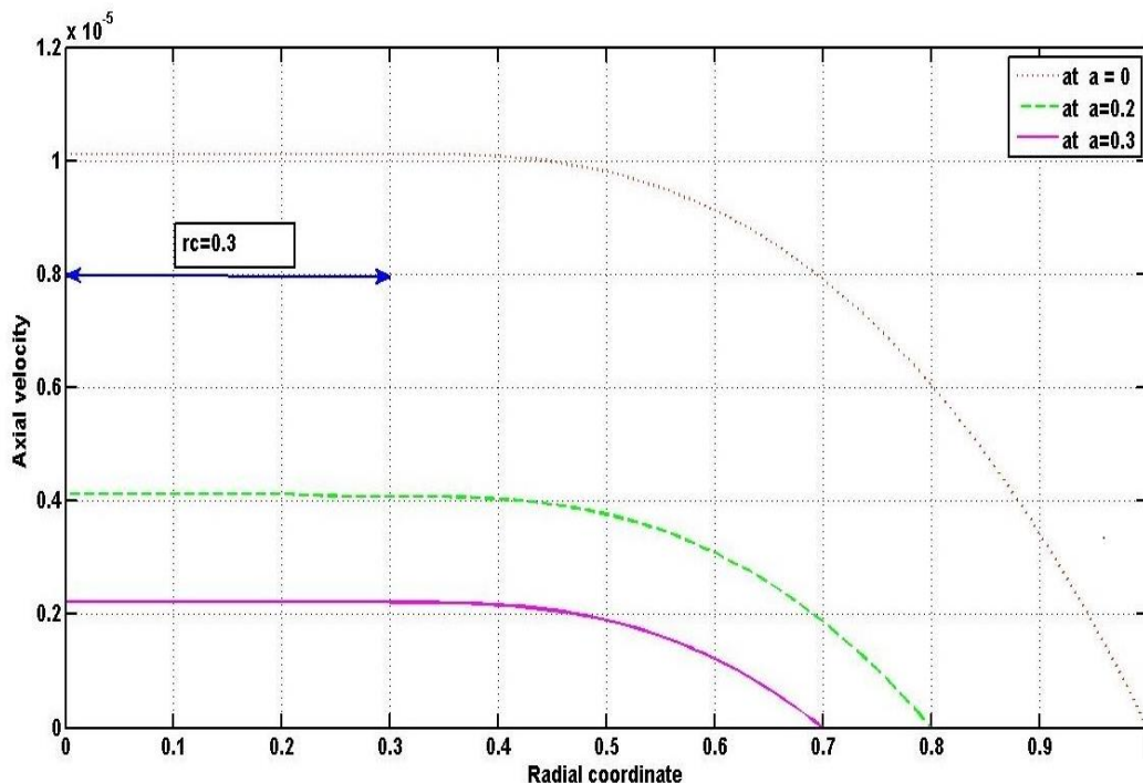
Figure 2. Variation of axial velocity with radial coordinate for different stenosis height a
