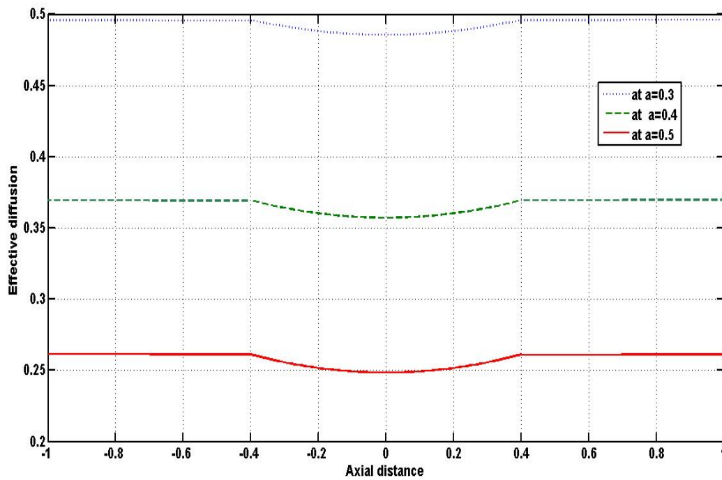
Figure 8: Variation of effective diffusion with axial distance for different stenosis height a
