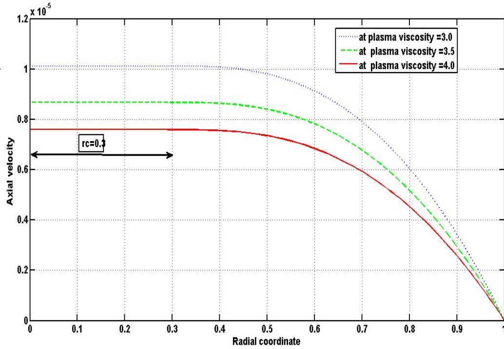
Figure 3. Variation of axial velocity with radial coordinate for different plasma viscosity \eta_1
