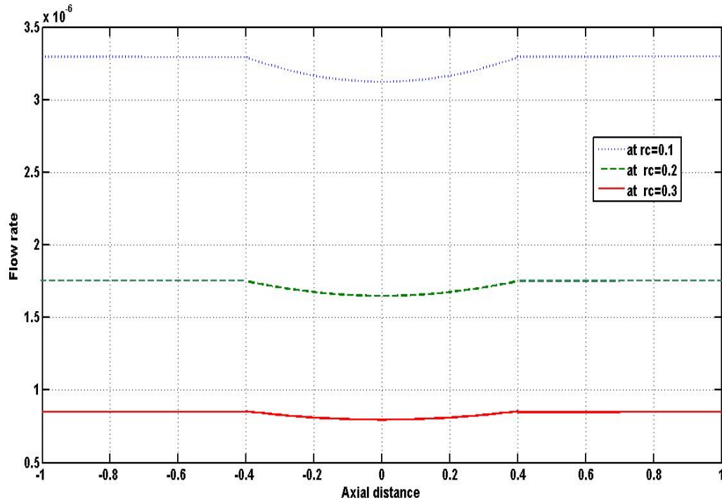
Figure 7. Variation of flow rate with axial distance for different rheological parameter r_c
