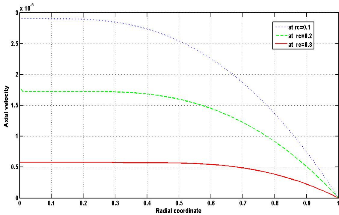
Figure 4. Variation of axial velocity with radial coordinate for different rheological parameter \tau_c
