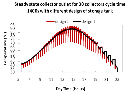
Figure 7. Collector outlet design 1 and design 2 at peak hours steady state
