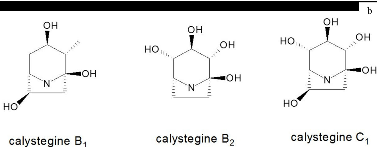
Figure 1b. Structures of the glycosidase-inhibitory alkaloids of the tropane found in the plant Ipomoea carnea .
