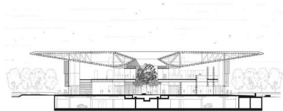
Fig.32: showing the section and the roof structure by the architects
