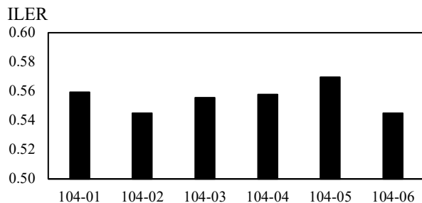
Fig. 8a: Installed Load Efficacy Ratio (ILER) for different arrangements of luminaries.
