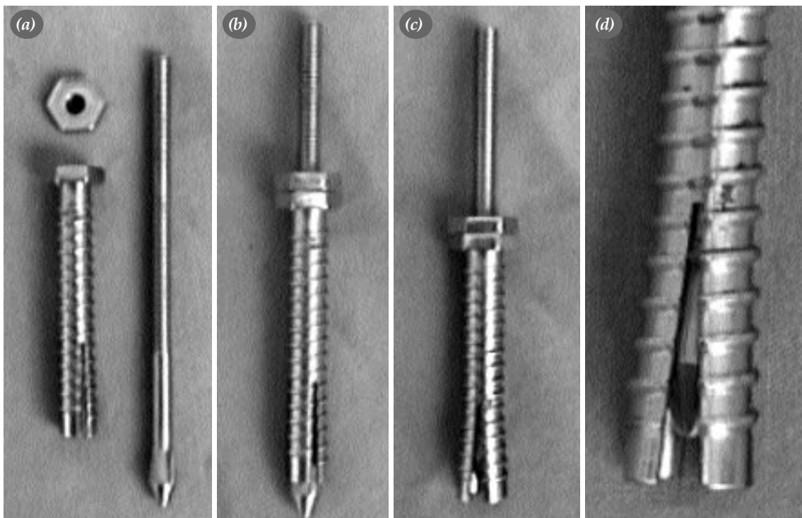
Figure 2. The views of expandable tipped pedicle screws type 1. The views of (a) separately (individually three parts), (b) composed and (c, d) expanded tip when the pin inside is pulled back.
