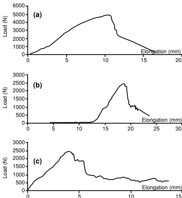
Figure 6. Load-elongation curves of (a) 6,5 mm and (b) 7 mm Alici type pedicle screws and (c) expandable pedicle screw type 2.
