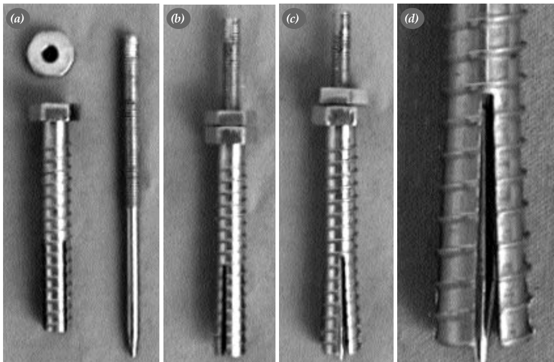
Figure 3. The views of expandable tipped pedicle screws type 2. The views of (a) separately (individually three parts), (b) composed and (c, d) expanded tip when the pin inside is moved to the tip (to the forward).
