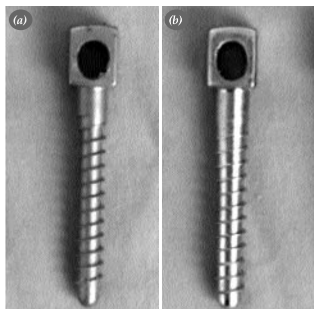
Figure 1. The views of Alici pedicle screws (a) 6.5 mm, and (b) 7 mm in diameter.
