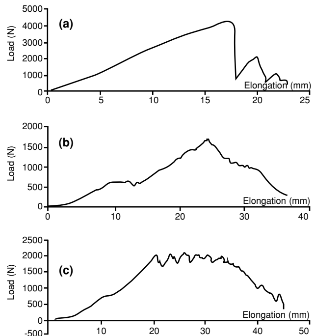
Figure 5. Load-elongation curves of (a) 6,5 mm and (b) 7 mm Alici type pedicle screws and (c) expandable pedicle screw type 1.
