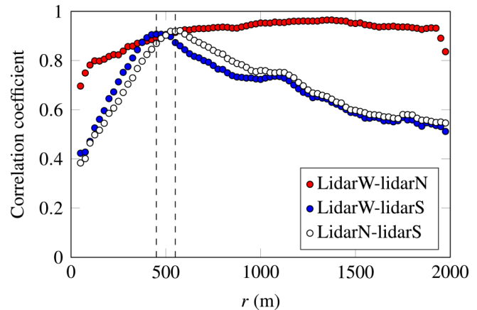
Figure 15. Pearson correlation coefficient between each pair of time series, at increasing distances from LidarW or LidarN. The dashed lines indicate the distance at which the correlation coefficient is largest for LidarW–LidarS and LidarN–LidarS.
