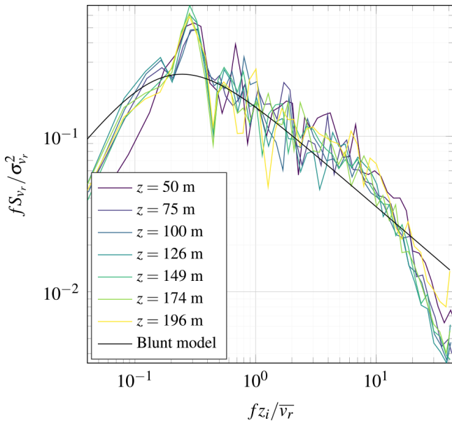
Figure 19. Power spectral density estimate of the velocity component v_r recorded on 25 October 2019 from 13:35 to 14:25 using beams parallel to the mean wind direction with an elevation angle of 4.9^\circ . The mean wind speed was \bar{v}_r \approx 14 \text{ m s}^{-1} at the different heights selected and z_i = 1153 \text{ m} .
