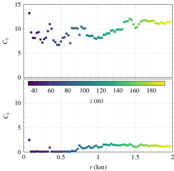
Figure 17. Decay parameters at increasing scanning distances (abscissa) and increasing heights (colour bar) obtained by fitting Eq. (7) to the co-coherence between LidarW and LidarN after correction for elevation and azimuth offsets.
