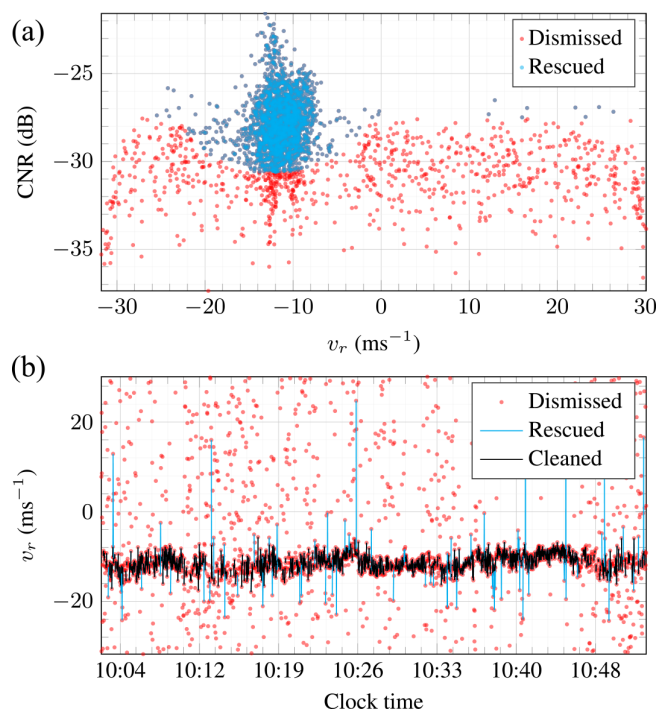
Figure 6. (a) Scatter plot of the CNR versus the along-beam velocity on 25 October 2019 from 10:03 to 10:52 for the range gate located 275 m away from the lidars. (b) Corresponding time series showing the dismissed and rescued samples using the Mahalanobis distance and the cleaned data after application of outlier analysis based on the median absolute deviation.
