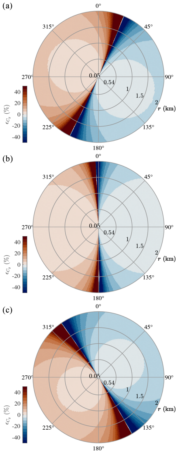
Figure 9. Relative error \epsilon_{C_y} on the Davenport decay coefficient C_y between LidarN and LidarW (a), LidarN and LidarS (b), and LidarW and LidarS (c), assuming an azimuth offset of -0.1^\circ for one of the two lidars selected. This relative error is independent on the value of C_y . The colour map was taken from Crameri (2018).
