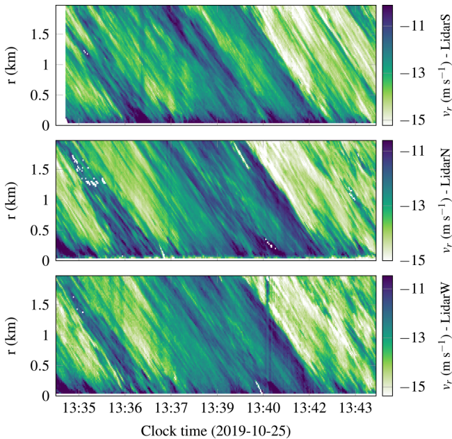
Figure 14. Along-beam velocity component simultaneously recorded on 25 October 2019 by the three scanning lidar instruments at every range gate.
