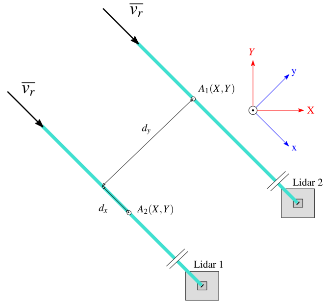
Figure 8. Schematic of the distances d_x and d_y defined by the two closest range gates for a given scanning distance.
