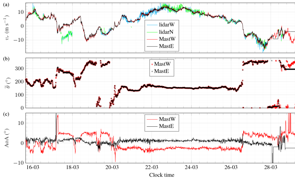
Figure 12. 10 min along-beam mean wind speed (a), mean wind direction \bar{\theta} (b) and mean angle of attack (AoA, c) recorded from 16 to 29 March 2020 on the northern side of Obrestad Lighthouse.
