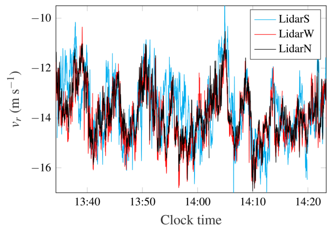
Figure 13. Along-beam velocity component recorded on 25 October 2019 by LidarN, LidarS and LidarW at r = 1975 \text{ m} .
