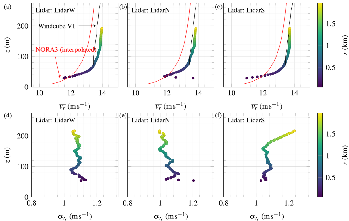
Figure 16. (a, b, c) Mean wind speed recorded along the beams of the scanning lidar units (scatter) superposed to the wind profile of the WindCube V1 and the NORA3 hindcast 3 km away from the coast (solid lines). (d, e, f) Standard deviation of the along-beam component at increasing distances and heights on 25 October 2019 from 13:35 to 14:25.
