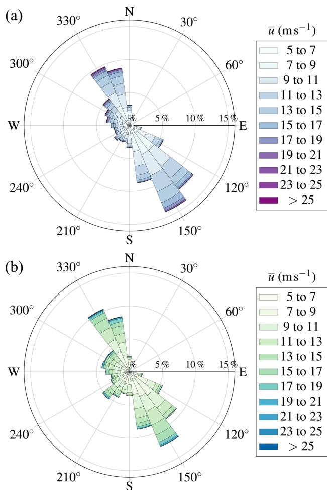
Figure 3. Wind roses computed using 10 min mean wind records from 1990 to 2020 (a) and from March 2019 to March 2020 (b), 10 m above the ground by the Obrestad Lighthouse weather station. Only samples associated with \bar{u} \geq 5 \text{ m s}^{-1} are considered for the sake of clarity.
