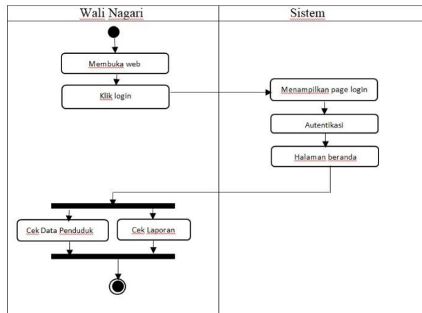
Gambar 7. Activity Diagram Wali Nagari
