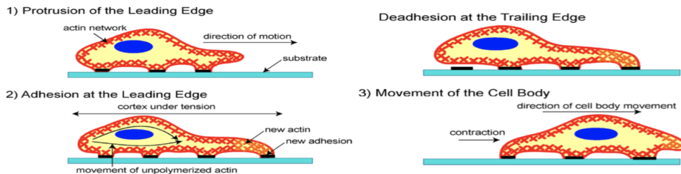
FIGURE 1. Scheme of cell crawling over a flat substrate [1]
