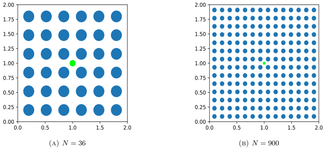
FIGURE 8. Domain \Omega = [0, 2] \times [0, 2] . Obstacles in blue, cell initial position in green. For case (a): \varepsilon = 0.01 , r_O = 0.1 , r = r_O/2 = 0.05 . For case (b): \varepsilon = 0.01 , r_O = 0.04 , r = r_O/2 = 0.02 .
