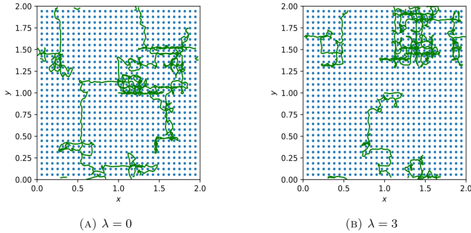
FIGURE 10. Particle's trajectories for N = 900 obstacles. Parameters: \alpha = 0 , \beta = 0 , \sigma = 1 , \lambda = 0 (10a) and \lambda = 3 (10b).
