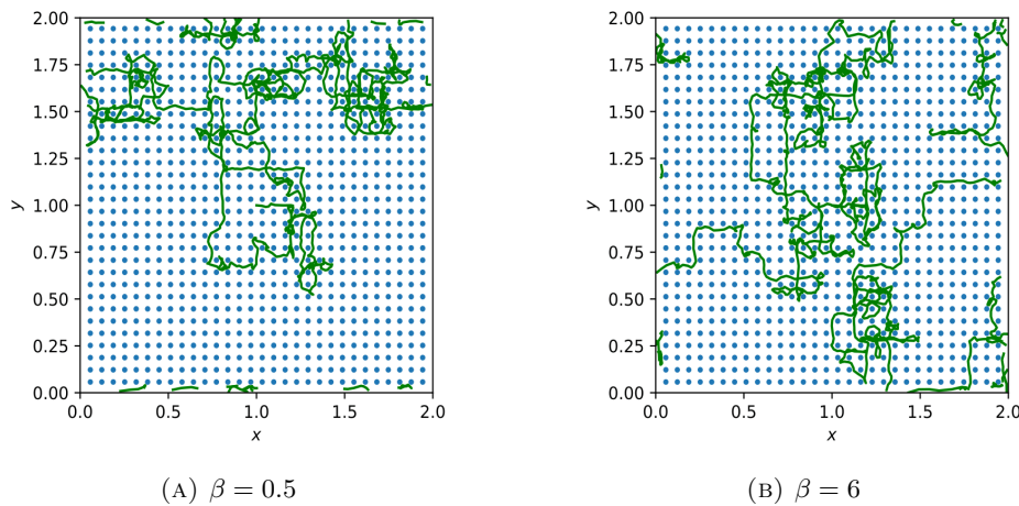
FIGURE 16. Particle's trajectories for N = 900 obstacles. Parameters: \alpha = 30 , \lambda = 1 , \sigma = 0.2 , \beta = 0.5 (16a) and \beta = 6 (16b).
