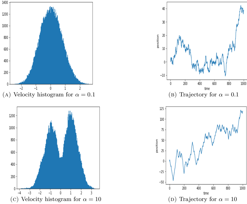
FIGURE 6. Histogram for the velocity V solution of Equation (6) (6a,6c) and cell trajectory (6b,6d) for h = 0.5 , \lambda = 1 , \gamma = c = \sigma = 1 , \beta = 0.1 , \alpha = 0.1 (6a,6b) and \alpha = 10 (6c,6d).
