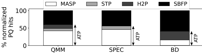
Fig. 12: Percentage of PQ hits provided by ATP (its constituent prefetchers) and SBFP.
