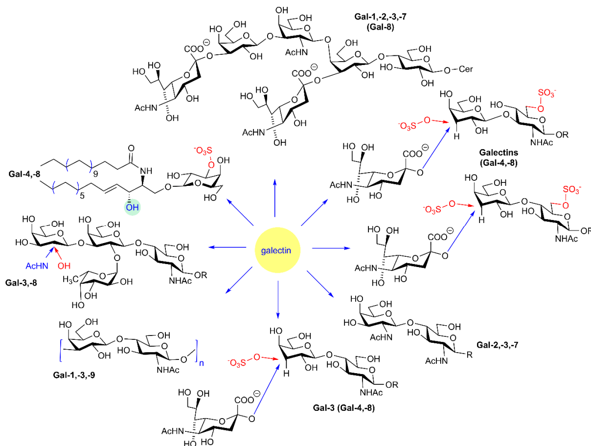
Figure 5. Illustrations of galectin binders from the class of natural \beta -galactosides and naming of examples of mammalian galectins with high affinity for a glycan, for example galectin-8 (Gal-8) for 3'-sulfated LacNAc and the hexasaccharide of ganglioside GD1a or galectins-1, -2, -3 and -7 (Gal-1, -2, -3 and -7) for the pentasaccharide of ganglioside GM1 (please see Figure 11 for examples of bioactivity of GM1 binding by these adhesion/growth-regulatory galectins).
