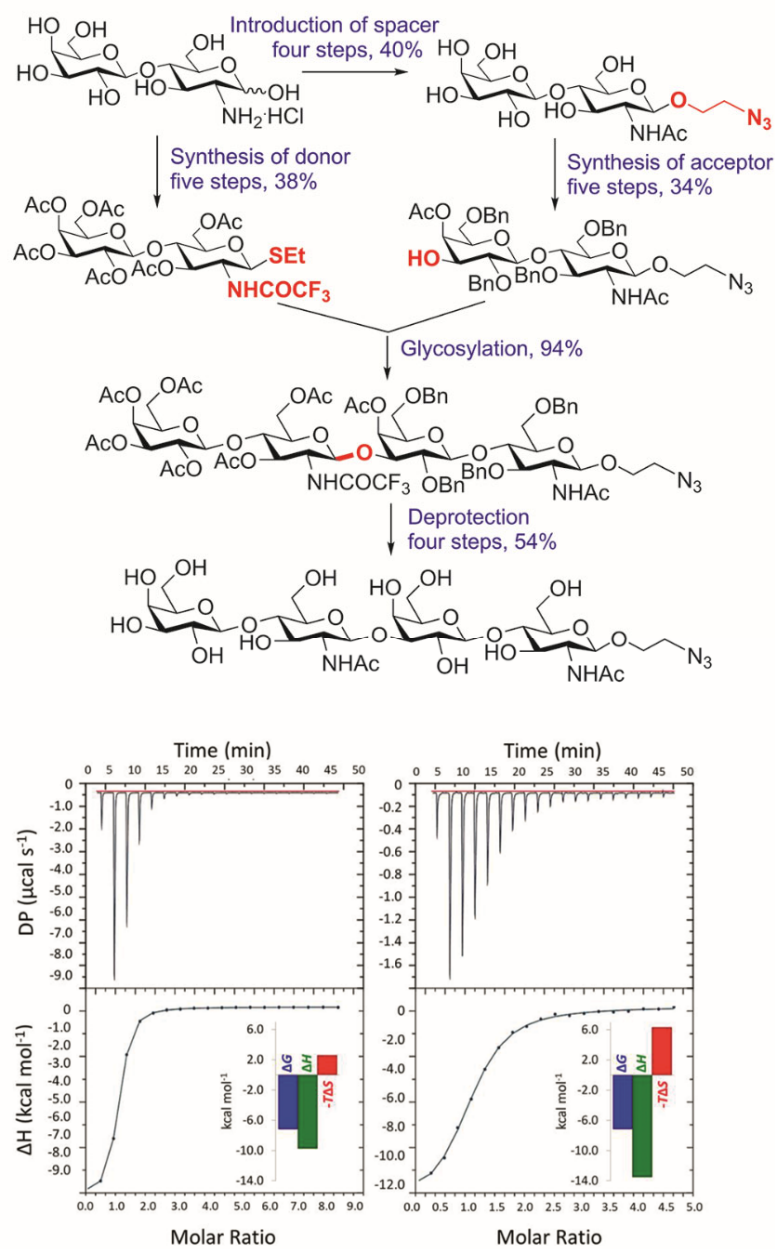
Figure 2. Overview on DiLacNAc synthesis (for details, please see Supplementary Material, Scheme S1) and the calorimetric titration profiles of its interaction with human galectin-3 in H 2 O (bottom, left) and D 2 O (bottom, right). For details, please see [63e] .
