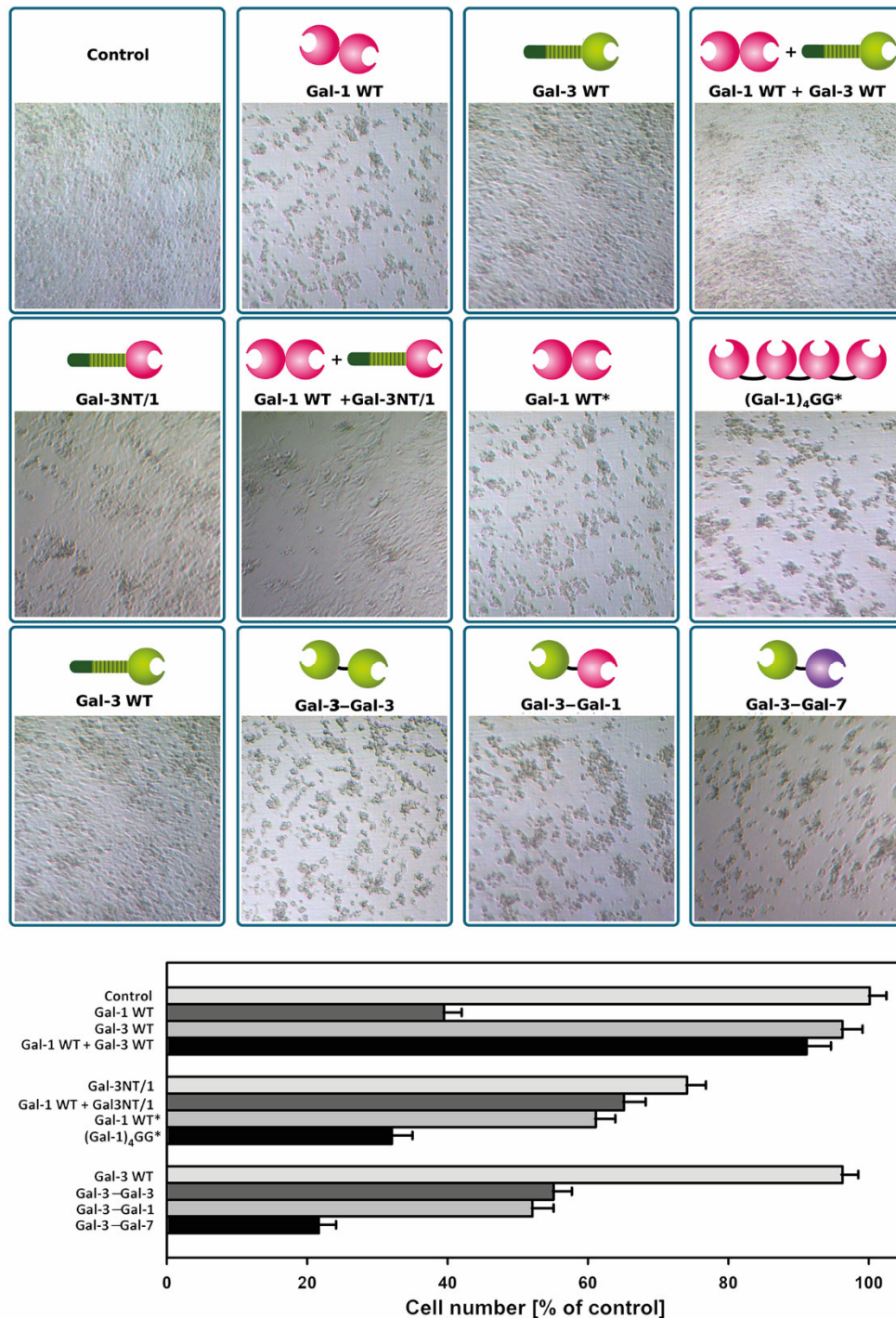
Figure 11. Effect of wild-type and of engineered human galectins on neuroblastoma cell (SK-N-MC) growth. Galectin architecture, microphotographs of representative cultures and a bar
