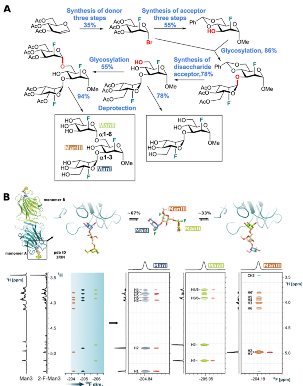
Figure 7. Overview of the synthesis of the trifluorinated N -glycan core trimannoside (for further information, please see Supplementary Material, Scheme 4) (A), the crystallographic information on trimannoside binding in two modes (PDB 1RIN) (B) and NMR-spectroscopical information on binding of the trifluoro-trimannoside (2F-Man3) by Pisum sativum (pea) agglutinin (C); from left to right: 1D ^1\text{H} of Man3, 1D ^1\text{H} 2F-Man3; 2D ^1\text{H} , ^{19}\text{F} TOCSYreF correlation spectrum; 2D ^1\text{H} , ^{19}\text{F} STD TOCSYreF spectra (strips) of 2F-Man3 in the bound state revealing
