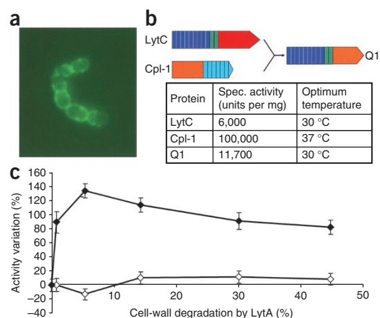
Figure 2 Localization of GFP-LytC, properties of Q1 chimeric protein, and differential behavior between LytC and Cpl-1. (a) Subcellular localization of LytC by fluorescence image of the GFP-LytC fusion protein added to the pneumococcal culture. (b) Schematic representation of the Q1 chimeric protein. The modular construction of the parental proteins is represented by different colors: red and orange for catalytic modules of LytC and Cpl-1, respectively; deep blue and green for repeats of the choline-binding motifs of LytC, and light blue for repeats of the choline-binding motifs of Cpl-1. The relevant enzymatic properties of the parental and chimeric proteins are presented. (c) Increase of in vitro LytC activity by the pretreatment of pneumococcal cell walls with small amounts of LytA added to cell walls before the action of LytC or Cpl-1.
