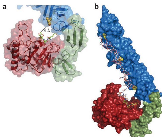
Figure 3 Proposed interaction between LytC and PG substrate attached to teichoic acid chains. (a) Details of the active site of LytC with the bound PG fragment (green sticks). Choline molecule attached to the site formed by repeats p7 and p8 is about 9 Å away from the PG bound to the active site. Loop L_c (residues 364–381) is labeled. (b) Computational model of PG-TA moiety bound to LytC active site based on the crystal structure of the LytC–choline–PG ternary complex and the NMR structure of a TA chain from S. pneumoniae R6 strain 15 . The docked choline moieties are represented as spheres.
