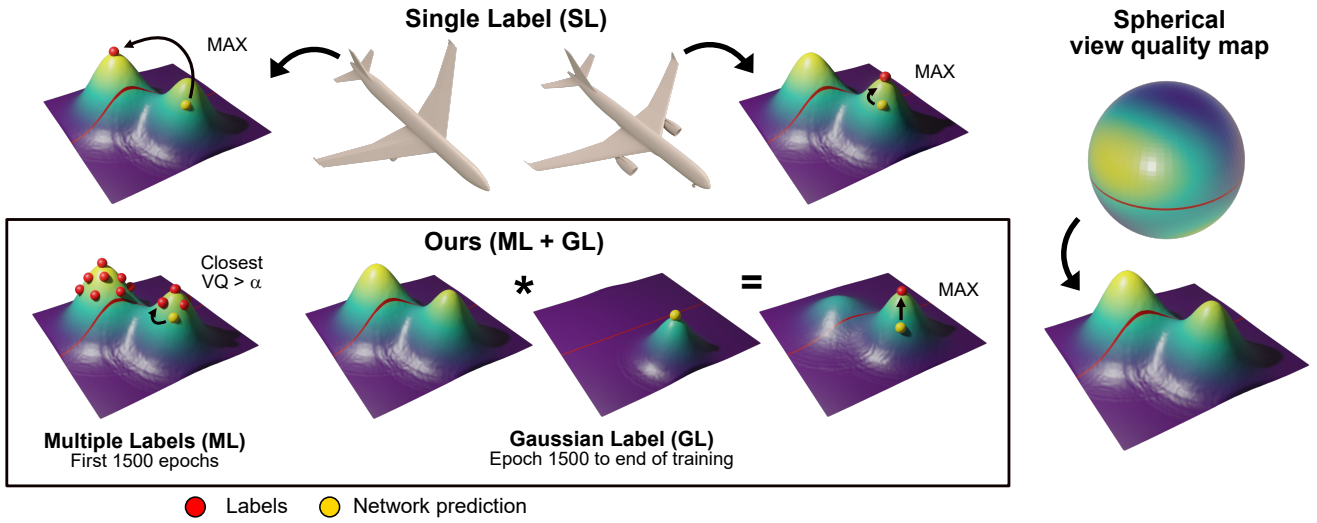
Figure 3: Dynamic label generation. Illustration of the proposed dynamic label generation technique for best viewpoint prediction, we use Mercator projections of the viewpoint sphere, as indicated on the right. Top: Best viewpoints are not necessarily unique, thus randomly choosing a maximum as label can create different labels for similar input models, which the network is unable to resolve. Bottom: To harmonize the label decision, we propose our two stage dynamic label generation. We first provide the network with multiple labels (ML) of high viewpoint quality and optimize towards the closest one. The labels typically form clusters in high quality areas, in which case the optimization tends to converge towards the boundary. To refine the predictions, we generate the label dynamically in a second stage (GL). The viewpoint quality distribution is weighted with a Gaussian centered at the current prediction and the maximum of the result is used as a label, which is typically a close local maximum, i.e., the maximum of the closest cluster. Both stages, ML and GL, provide more similar labels for similar input.
