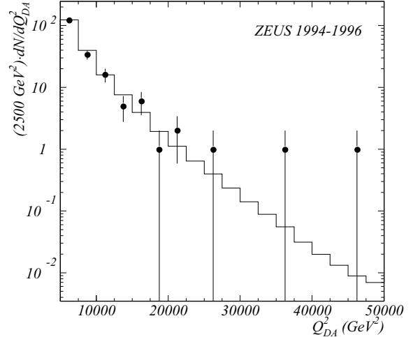
Fig. 3. The Q_{DA}^2 distribution of the observed events (full dots), compared to the Standard Model e^+p NC expectation (histogram). The error bars on the data points are obtained from the square root of the number of events in the bin
