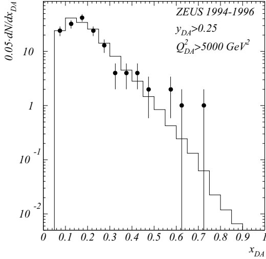
Fig. 2. The x_{DA} distribution of the observed events with the cuts shown (full dots), compared to the Standard Model e^+p NC expectation (histogram). The error bars on the data points are obtained from the square root of the number of events in the bin
