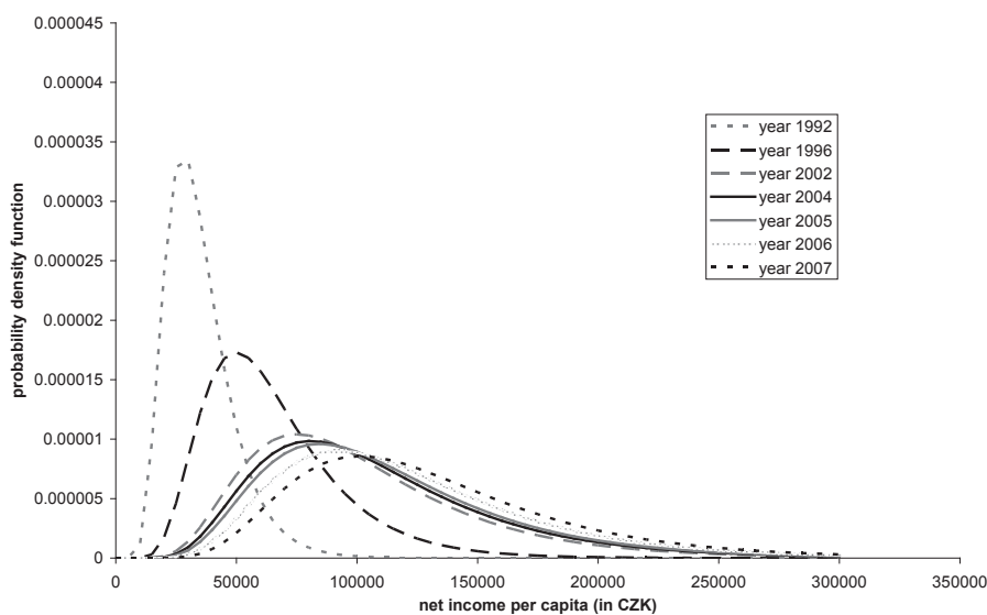
Figure 6: Estimated lognormal densities for annual net per capita income (CZK) for 1992, 1996, 2002, 2004–2007 (maximum likelihood method).
