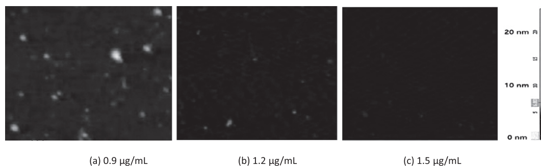
Fig. 7. Effect of GBP at different concentrations on amyloid beta. Representative AFM images of adsorbed 20 \mu M amyloid beta (1–42) oligomers prepared by HFIP protocol (Mica surfaces 3 \times 3 \mu\text{m} ) were visualized after 24 h incubation with preparations (images in 3 \times 3 \mu\text{m} , 24 h incubation).
