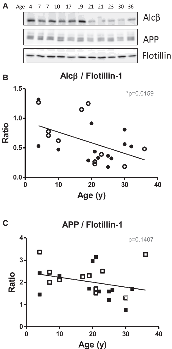
Fig. 3. Age-dependent changes of Alc \beta and APP expression in the monkey brain. (A) Protein levels of Alc \beta and the APP in the temporal cortices of various aged cynomolgus monkeys. Brain lysates (10 \mu g protein) were analyzed by immunoblotting with anti-Alc \beta and anti-APP antibodies, along with the anti-flotillin-1 antibody. (B, C) Band densities of Alc \beta and APP were quantified and normalized against the amount of flotillin-1. Relative ratios for Alc \beta (B) and APP (C) were plotted versus age. Open symbols indicate samples shown in panel (A). Statistical analysis was performed using Pearson's correlation, and significance with P -value is indicated. Age (y) indicates years old. Abbreviations: APP, amyloid \beta protein precursor; Alc \beta , A \beta .
