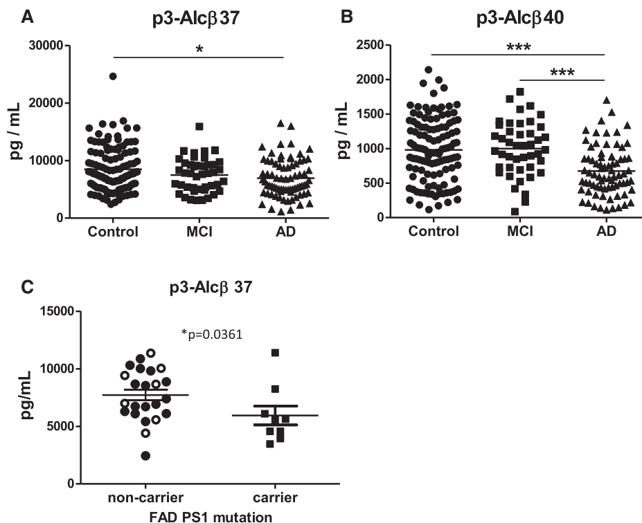
Fig. 4. Comparisons of the p3-Alc \beta levels in the CSF of patients with sporadic AD, patients with MCI, and nondemented subjects, and in the CSF between subjects with or without PSEN1 gene mutations. CSF p3-Alc \beta 37 (A) and p3-Alc \beta 40 (B) levels were compared among non-AD controls (n = 117), patients with MCI (n = 44) and patients with AD (n = 76) subjects. The summary of subjects and results is shown in Tables 1, and Supplementary Tables 1 and 2. Statistical examination was performed with the Kruskal-Wallis test, and P -values are indicated (* P < .05; *** P < .001). (C) p3-Alc \beta 37 levels in CSF were compared between subjects with PSEN1 mutations (carrier, n = 9, closed square) and those without PSEN1 mutations (noncarrier, n = 23). The summary of subjects is shown in Supplementary Table 3. Noncarriers (average age 42) include family members of carriers (n = 16, closed circle) and subjects carrying APP gene mutation (n = 7, open circle). Statistical examination was performed by Mann-Whitney U test, and P -values are shown (* P = .0361). Carriers include seven nondemented (CDR 0) subjects, whereas noncarriers include 19 nondemented (CDR 0) subjects. Error bars indicate \pm S.E. Abbreviations: Alc \beta , Alcadin \beta ; AD, Alzheimer's disease; CSF, cerebrospinal fluid; MCI, mild cognitive impairment; APP, amyloid \beta protein precursor; CDR, clinical dementia rating; S.E., standard error.
