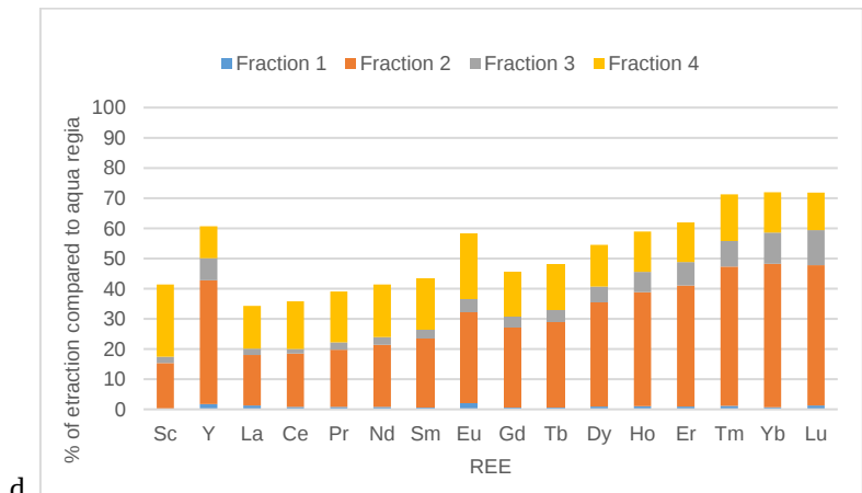
Figure 7: Sequential extraction of REE in ESS soil samples a) E4, b) E258 (where Eu in the fraction 4 was an outlier), c) E331, d) E344 using the 4-step Mittermüller et al. method [67] (see section 4.4.2 for the detailed methods)
