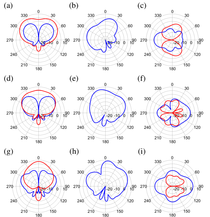
Fig. 15. Simulated radiation patterns of co-designed two broadside tri-modal patch MIMO array with E -phi (red), and E -theta (blue). Port 1 at 3.7 GHz is (a)-(c), port 1 at 4.1 GHz is (d)-(f), and port 10 at 5.5 GHz is (g)-(i). The xz -plane is in (a), (d) and (g); the yz -plane is in (b), (e) and (h); and the xy -plane is in (c), (f) and (i).
