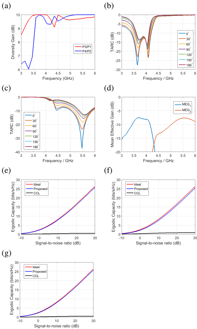
Fig. 12. MIMO performance of co-designed two broadside tri-modal patch antennas: (a) diversity gain; (b) TARC of port 1 (c) TARC of port 2; (d) MEG; (e) ergodic capacity at 3.7 GHz; (f) ergodic capacity at 4.1 GHz; (g) ergodic capacity at 5.5 GHz.
