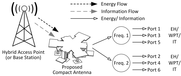
Fig. 1. Receiver schematic with dual-band energy and data transmission enabled.
