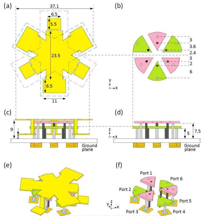
Fig. 7. Geometry of proposed co-designed two broadside tri-modal patch antennas (units: mm): (a) plan view; (b) plan view without radiator; (c) side view; (d) side view without radiator; (e) perspective view; and (f) perspective view without radiator.
