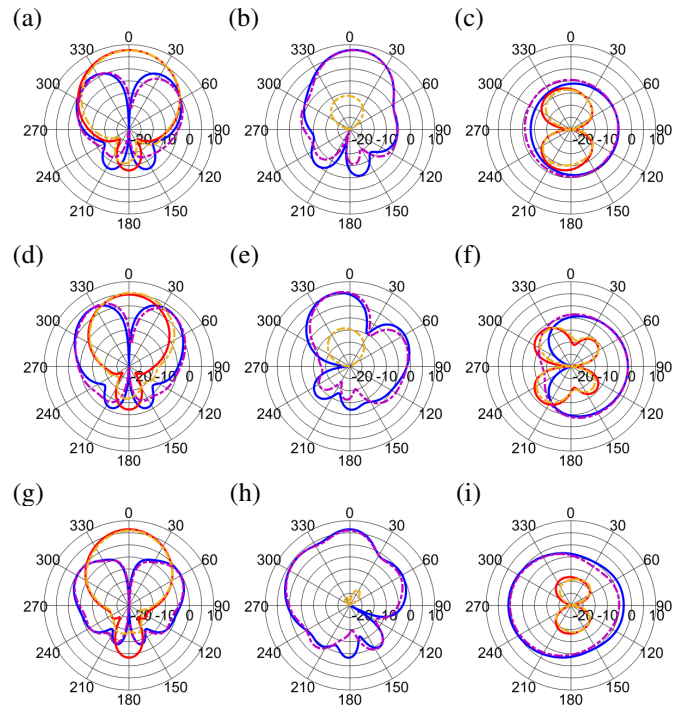
Fig. 11. Radiation patterns of co-designed two broadside tri-modal patch antennas with simulation (solid), measurement (dash-dot), E -phi (red/ orange), and E -theta (blue/ violet). Port 1 at 3.7 GHz is (a)-(c), port 1 at 4.1 GHz is (d)-(f), and port 4 at 5.5 GHz is (g)-(i). The xz -plane is in (a), (d) and (g); the yz -plane is in (b), (e) and (h); and the xy -plane is in (c), (f) and (i).
