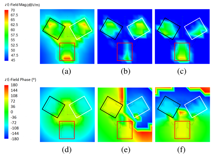
Fig. 4. The z -directed characteristic E-fields at 0.2 mm below the top snowflake patch in [24]: amplitude distribution of the first three modes at 5.5 GHz correspond to (a)–(c); phase distribution of the first three modes at 5.5 GHz correspond to (d)–(f).
