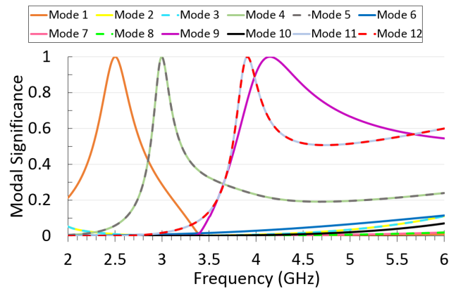
Fig. 3. Modal significance of broadside tri-modal patch antenna in [24].
