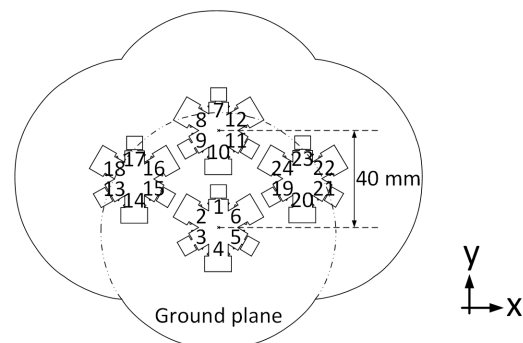
Fig. 13. Geometry of four elements co-designed two broadside tri-modal patch MIMO array.
