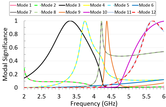
Fig. 6. Modal significance of proposed antenna structure with all six probes replaced by shorts.
