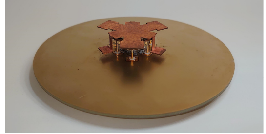
Fig. 8. Prototype of co-designed two broadside tri-modal patch antenna.
