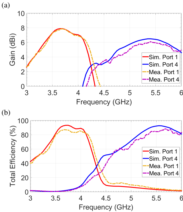
Fig. 10. Radiation performance of co-designed two broadside tri-modal patch antennas: (a) gains of ports 1 and 4; (b) efficiencies of ports 1 and 4.
