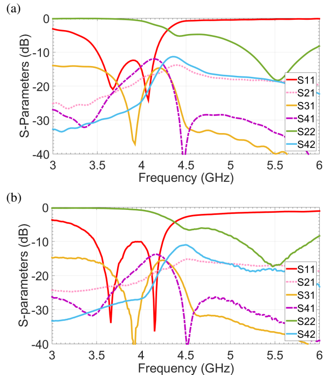
Fig. 9. S -parameters of co-designed two broadside tri-modal patch antennas: (a) simulation; (b) measurement.
