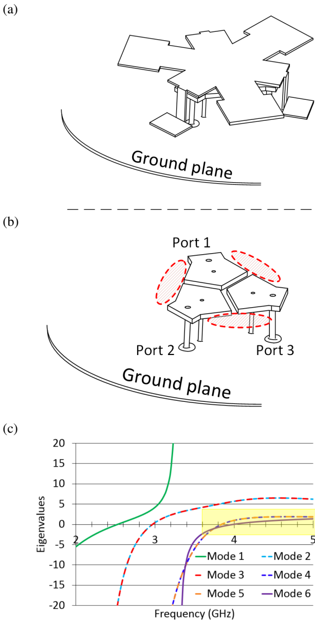
Fig. 2. Broadside tri-modal patch antenna in [24]: (a) overall structure; (b) capacitive loading plates with shorting pins; (c) eigenvalues (first six modes).
