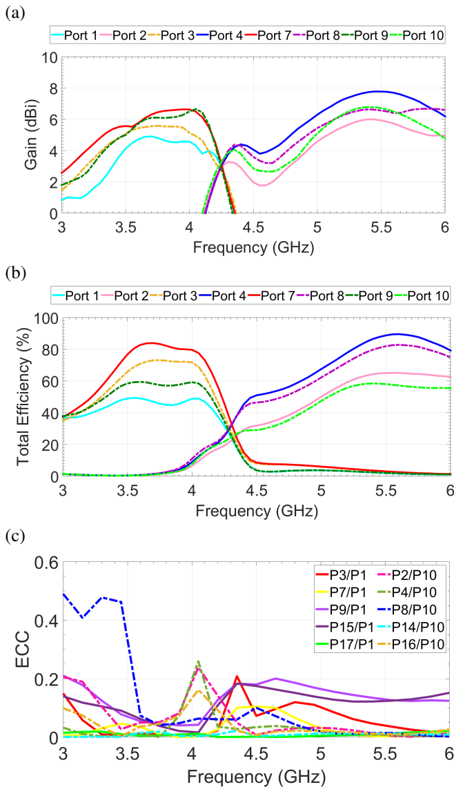
Fig. 16. Simulated radiation performance of co-designed two broadside tri-modal patch MIMO array: (a) gain; (b) efficiency; (c) envelope correlation coefficient.
