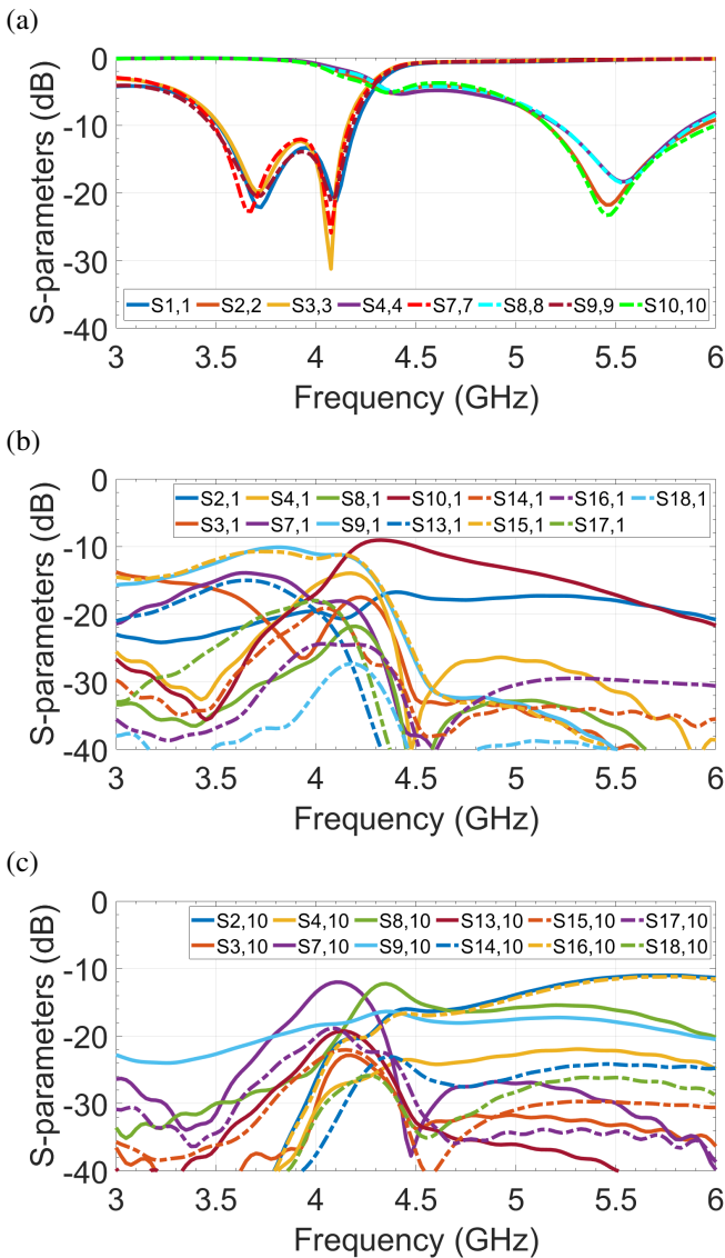
Fig. 14. Simulated S -parameters of co-designed two broadside tri-modal patch MIMO array: (a) reflections; (b) mutual couplings w.r.t. port 1; (c) mutual couplings w.r.t. port 10.
