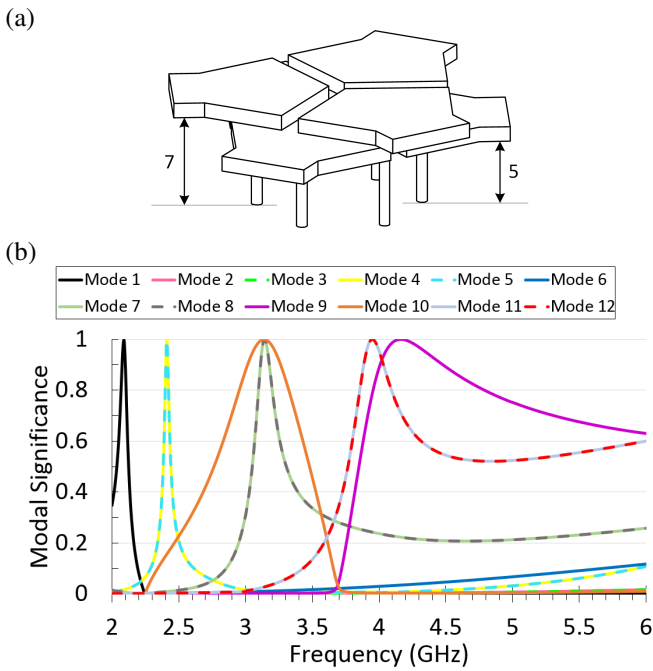
Fig. 5. Broadside tri-modal patch antenna in [24] with newly added capacitive loading plates: (a) geometry of six capacitive loading plates (units: mm); (b) modal significance.
