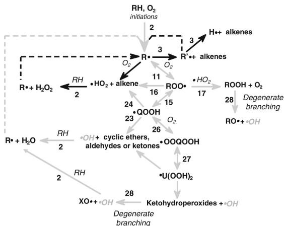
Figure 1.2: A simplified scheme for the mechanism of alkane oxidation. Reactions plotted in gray are important at low temperature (below 900 K), those in black at high temperature [21].
