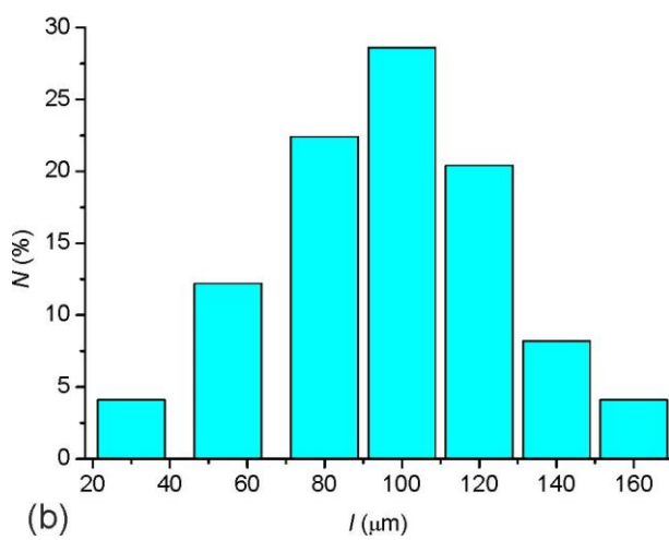
Fig. 3. (a) Microphotograph of the HANL fragment in crossed polarizers (shown by arrows) and (b) statistical distribution of the SDL lengths in the ensemble.
