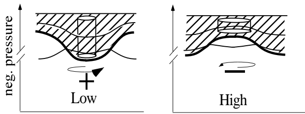
Figure 1. Stretching/shrinking of a tube of air in the lower stratosphere associated with a surface low/high pressure system [Hoskins et al. , 1985]. Stratospheric air (high potential vorticity) is hatched, the tropopause is given as a thick line, potential temperature surfaces as thin lines and \pm indicate sense of vorticity.
