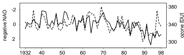
Figure 4. Total ozone (solid line, DJFM mean, in Dobson units) over Arosa and normalized NAO index (dashed line), scaled with -1.0 , based on pressure data from Iceland and Azores for the period 1932 to 1996. Compare to Figure 2 Panel C.
