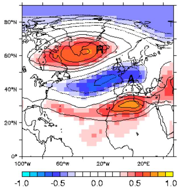
Figure 3. Cross correlation map (in colors) between winter mean (December to March) tropopause pressure and NAO index both derived from NCEP reanalysis data for the period 1958 to 1998. Only correlation coefficients above/below \pm 0.3 are shown. Contours indicate tropopause pressure variation associated with +1 SD in NAO index. Contour interval is 2 hPa, zero line omitted. (A) location Arosa and (R) location Reykjavik.
