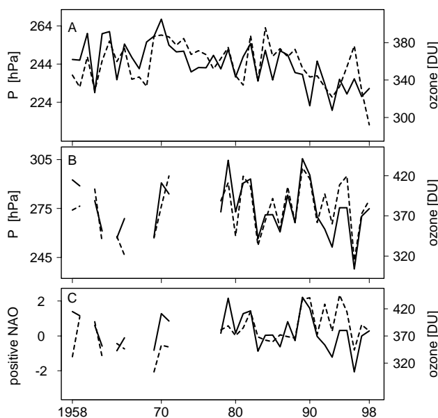
Figure 2. Panel A: February-March (FM) mean total ozone (solid line, in Dobson units) and tropopause pressure derived from NCEP reanalysis data (dashed line, in hPa) for the period 1958 to 1998, over Arosa, Switzerland. Panel B: As Panel A, but for Reykjavik, Iceland. Panel C: As Panel B but December to March means, and instead tropopause pressure with NAO index (dashed line) based on NCEP reanalysis data.
