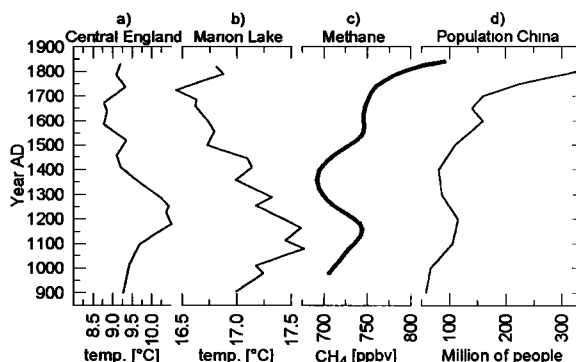
Fig. 3: Comparison between our data and historical records. a) Mean annual temperature of Central England [Lamb, 1977]. b) Growing season temperature from Marion Lake, Michigan [Bernabo, 1981]. c) Methane smoothed spline, this study. d) Population of China [McEvedy and Jones, 1979].
