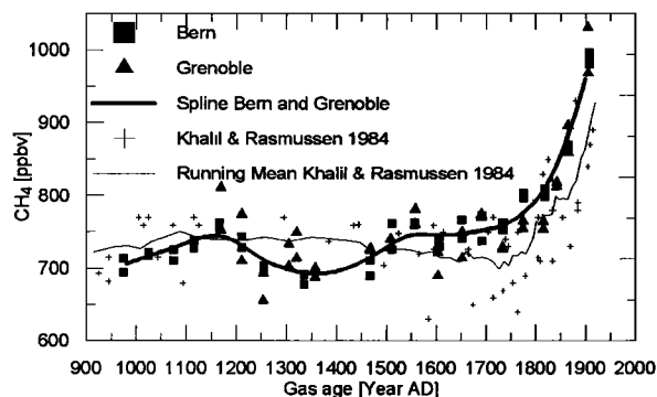
Fig. 2: Methane records versus the mean gas age. Squares and triangles from this study (squares: results from Bern; triangles: results from Grenoble) Thick solid line: Smoothed spline through the Bern and Grenoble data. Crosses: Results from various ice cores [Khalil and Rasmussen, 1984] corrected to Greenland concentration level. The mean gas age was recalculated after Schwander and Stauffer [1984]. Thin solid line: Running Mean of 9 data points.
