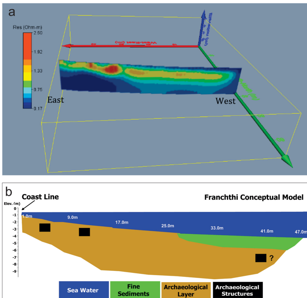
Fig. 11. Bay of Kildaha, Franchthi sector: a) 2-D resistivity distribution along a single ERT line; b) simplified conceptual model of the main stratigraphic units interpreted through the 2-D ERT models (direction east–west). The direction of the profiles is from east to west and the axis scale represents the distance and depth in metres.
