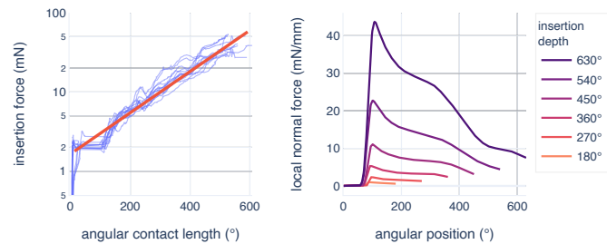
Fig. 4. Left: Insertion forces for parallel insertions increase exponentially with the angular contact length between the electrode array and the lateral wall. The graph shows 12 experiments with 7 dummies (0° mediolateral and basoapical at 0.33 mm/s, model B). The red line indicates the best fit according to (1). Right: Estimation of the line load resulting from the normal force at different angular depths of insertion according to (4).
