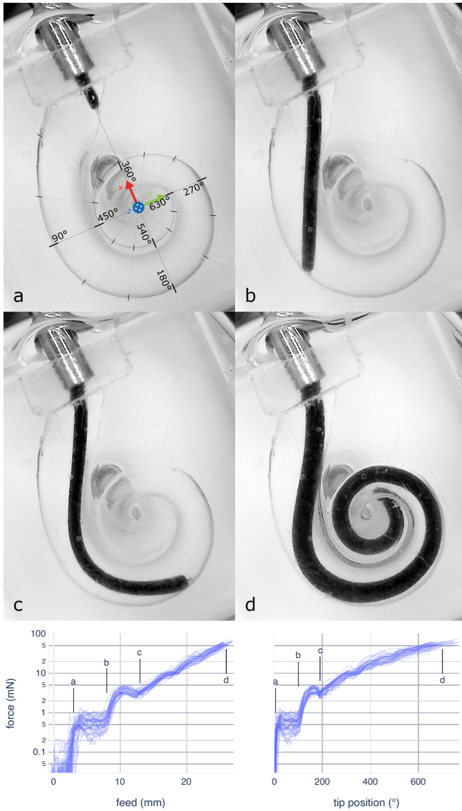
Fig. 2. Top: Images for a moderately angled insertion (20° mediolateral, 20° basoapical). a: First contact with modiolus wall, b: contact with lateral wall, c: Array bows outwards to the lateral wall, d: Full insertion. Bottom: Insertion forces as a function of the linear feed and angular insertion depth, respectively. The graph shows 39 repetitions with 7 dummies inserted at 0.33 mm/s into model B . For reference, the angular insertion depth is indicated on the first image.
