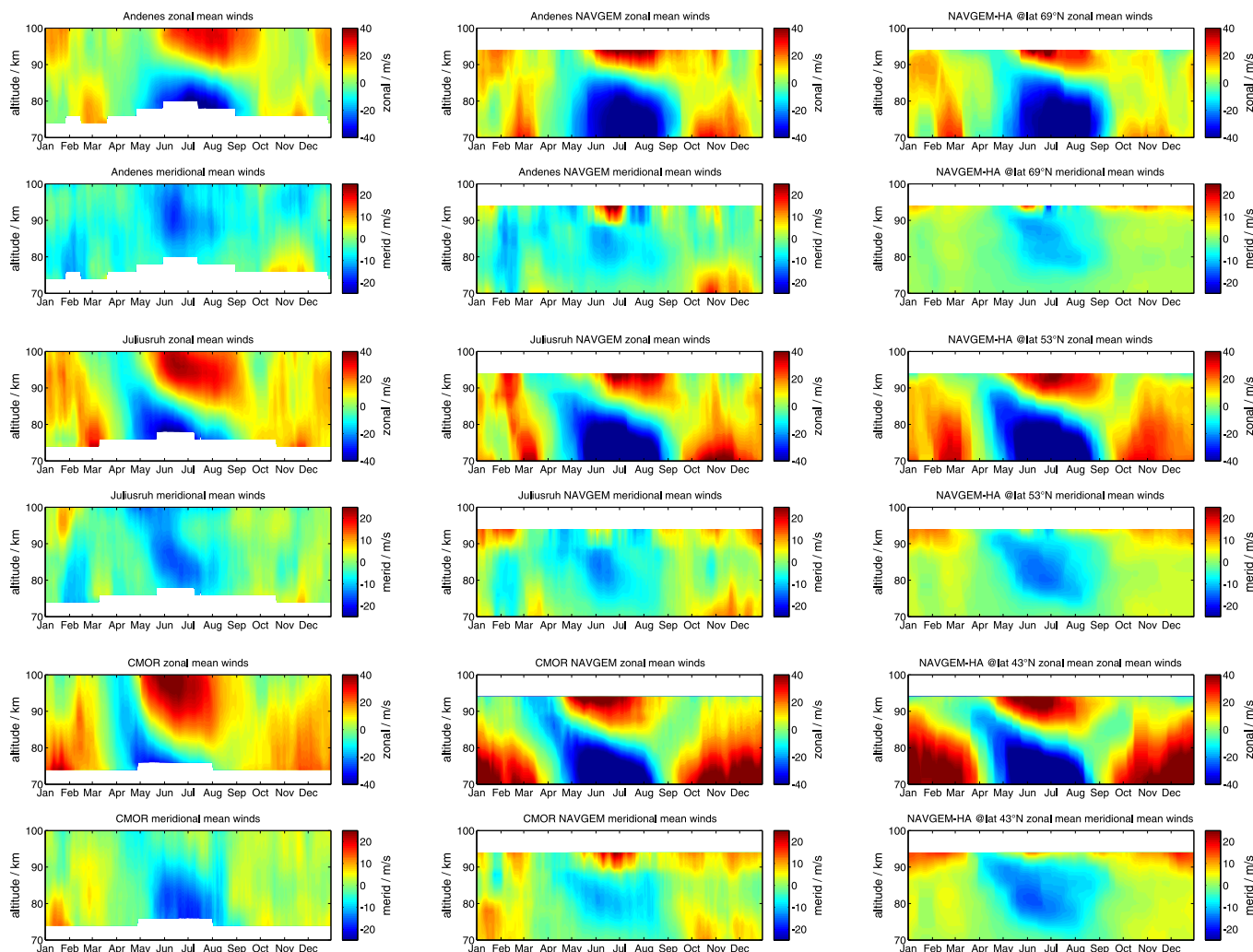
Figure 1. Comparison of mean winds above Andenes, Juliusruh and Tavistock (CMOR) using a 30-day running median with periodic boundary condition. The left panel shows the meteor radar observations. The central panel shows the NAVGEM-HA reanalysis fields for the same locations and periods. The right panel displays the zonal mean zonal and meridional winds for each latitude.
