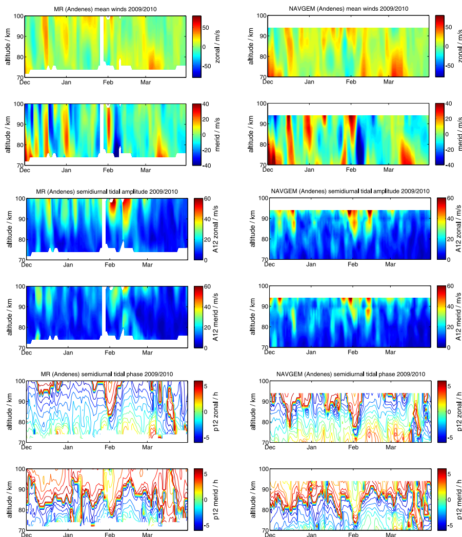
Figure 6. Comparison of meteor radar observations and NAVGEM-HA above Andenes during the winter 2009/10 for daily mean zonal and meridional winds (upper two panels), semidiurnal tidal zonal and meridional amplitude (middle panels) and semidiurnal tidal phases (lower two panels).
