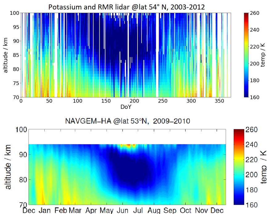
Figure 2. Comparison of mean temperatures above Kühlungsborn. The upper panel shows the temperatures derived from the potassium lidar. The lower panel shows the NAVGEM-HA reanalysis field for the same location.
