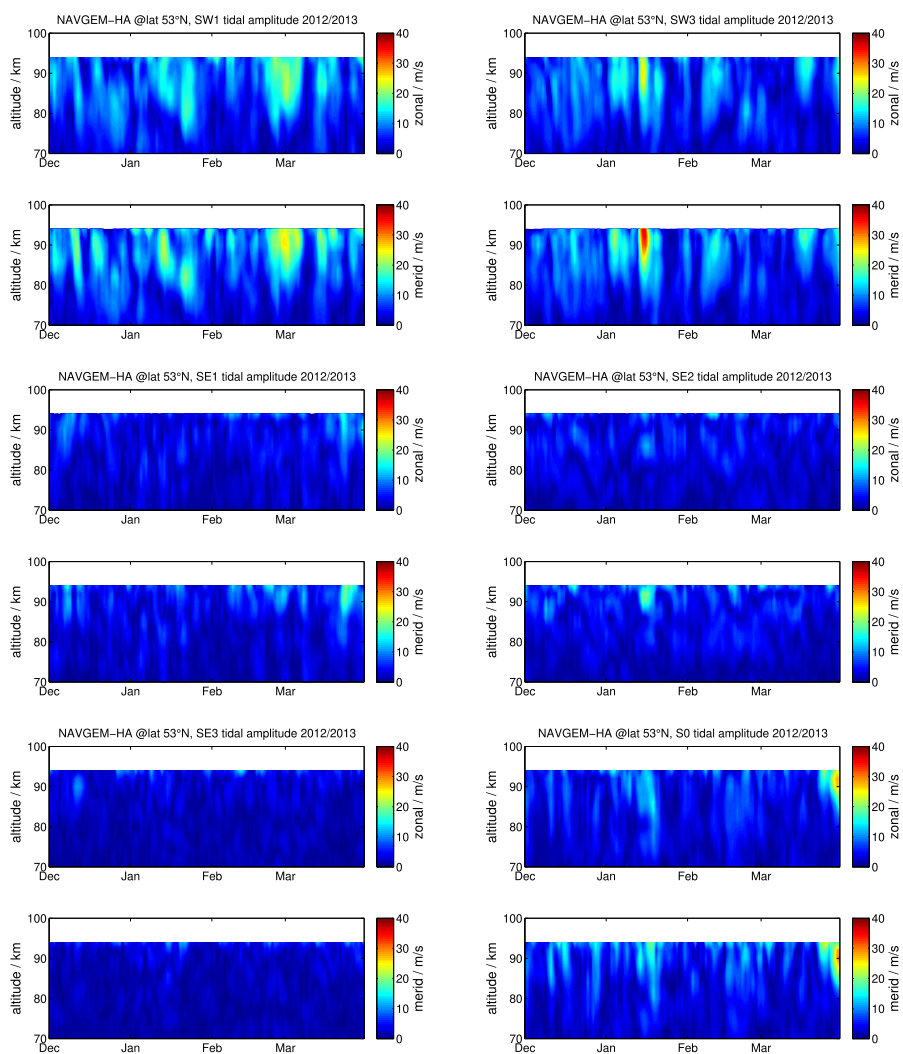
Figure A4. The same as Fig. A1 but above Juliusruh and for the winter 2012/2013.
