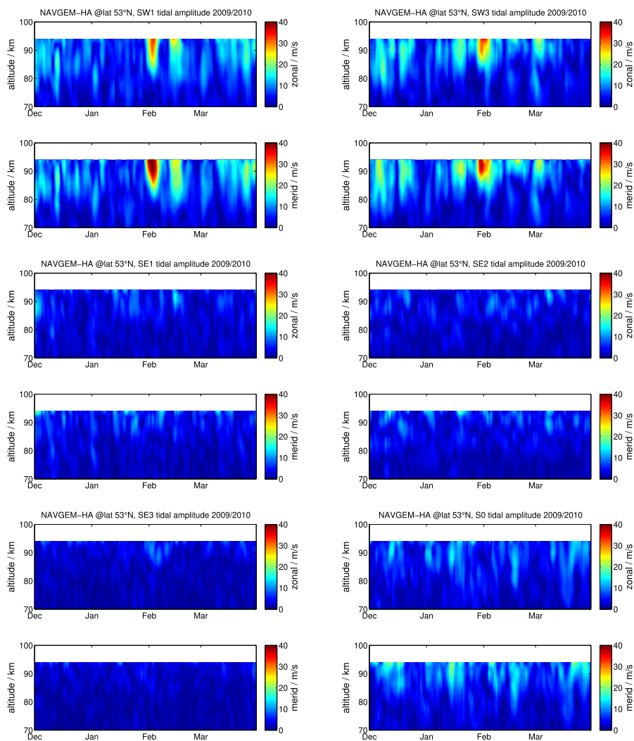
Figure A3. The same as Fig. A1 but above Juliusruh and for the winter 2009/2010.
