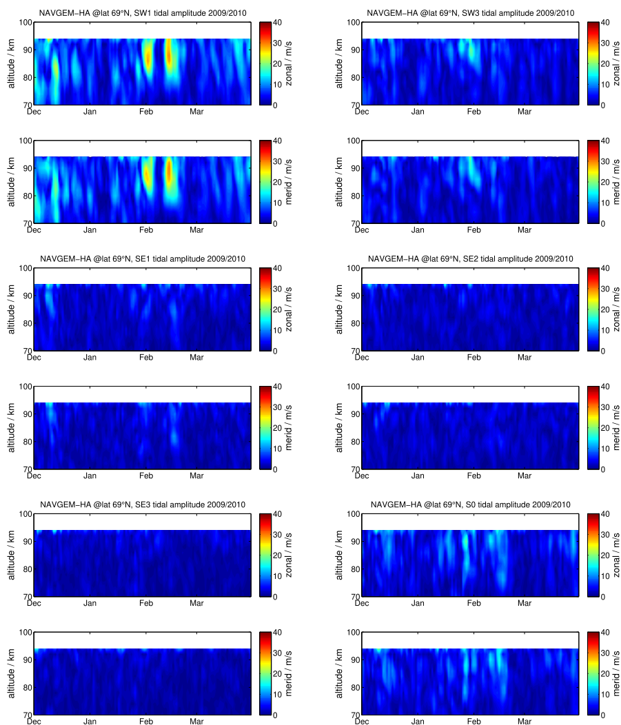
Figure A1. Non-migrating tides derived from global NAVGEM-HA winds above Andenes during the winter 2009/10 for SW1 and SW3 (upper two panels), SE1 and SE2 (middle panels), and SE3 and S0 (lower two panels) tidal components.
