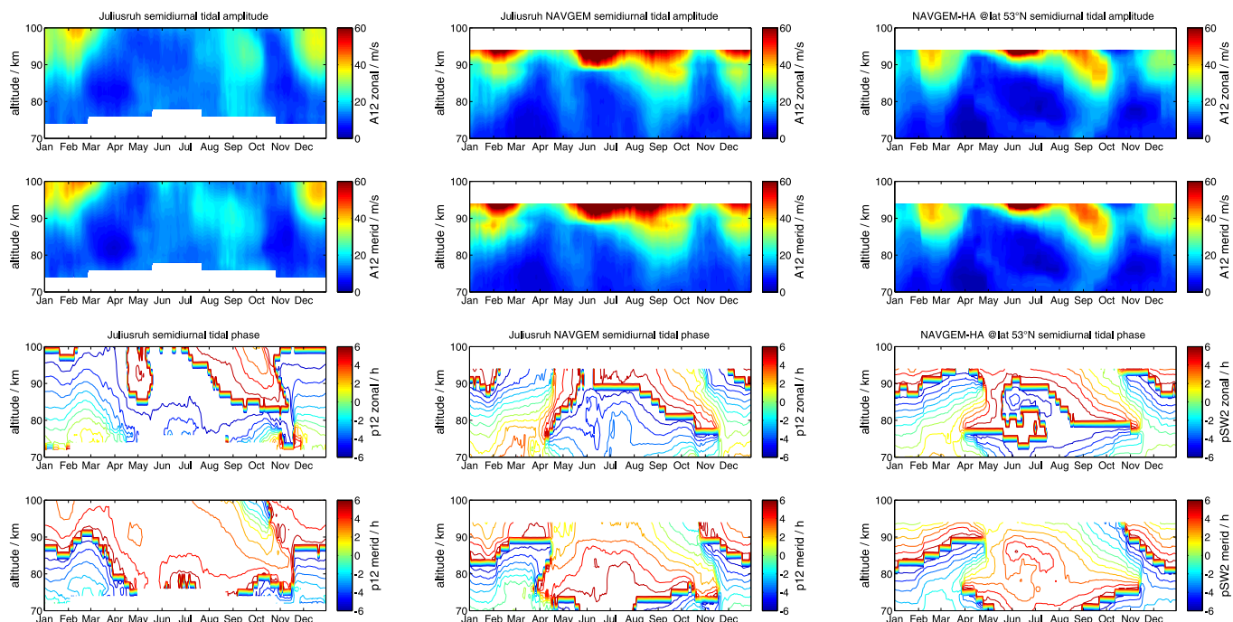
Figure 4. Comparison of semidiurnal seasonal amplitude and phase tidal climatology using a 30-day running median with periodic boundary condition. The left panels show the meteor radar observations above Juliusruh (54.3° N, 13° E). The central panels show the NAVGEM-HA reanalysis fields for the same period. The right panels visualize the zonal mean tidal amplitude and phase of the SW2.
