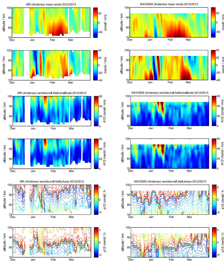
Figure 9. Comparison of meteor radar observations and NAVGEM-HA above Andenes during the winter 2012/13 for daily mean zonal and meridional winds (upper two panels), semidiurnal tidal zonal and meridional amplitude (middle panels) and semidiurnal tidal phases (lower two panels).
