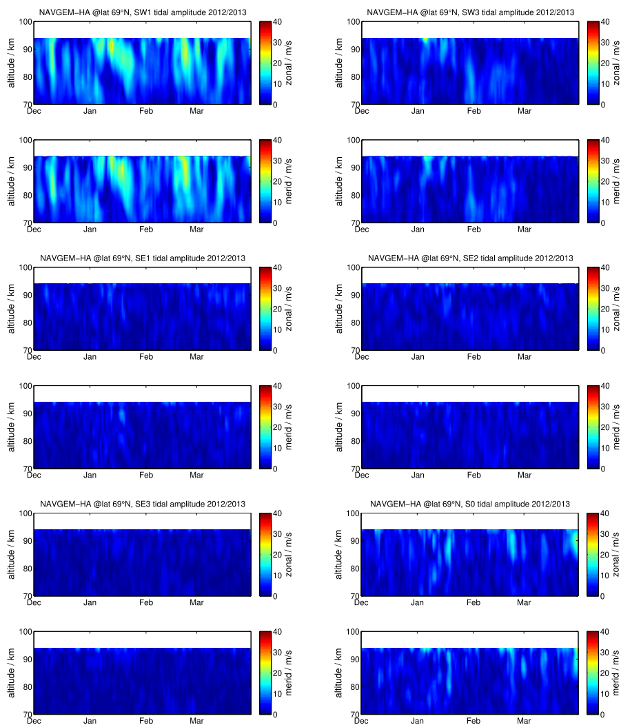
Figure A2. The same as Fig. A1 but for the winter 2012/2013.
