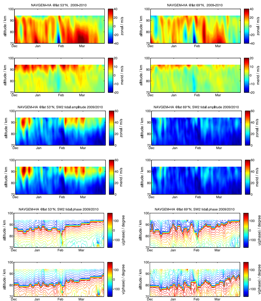
Figure 8. Comparison of global NAVGEM-HA above Andenes and Juliusruh during the winter 2009/10 for daily zonal mean zonal and meridional winds (upper two panels), zonal mean semidiurnal tidal zonal and meridional amplitude (middle panels) and zonal mean semidiurnal tidal phases (lower two panels).
