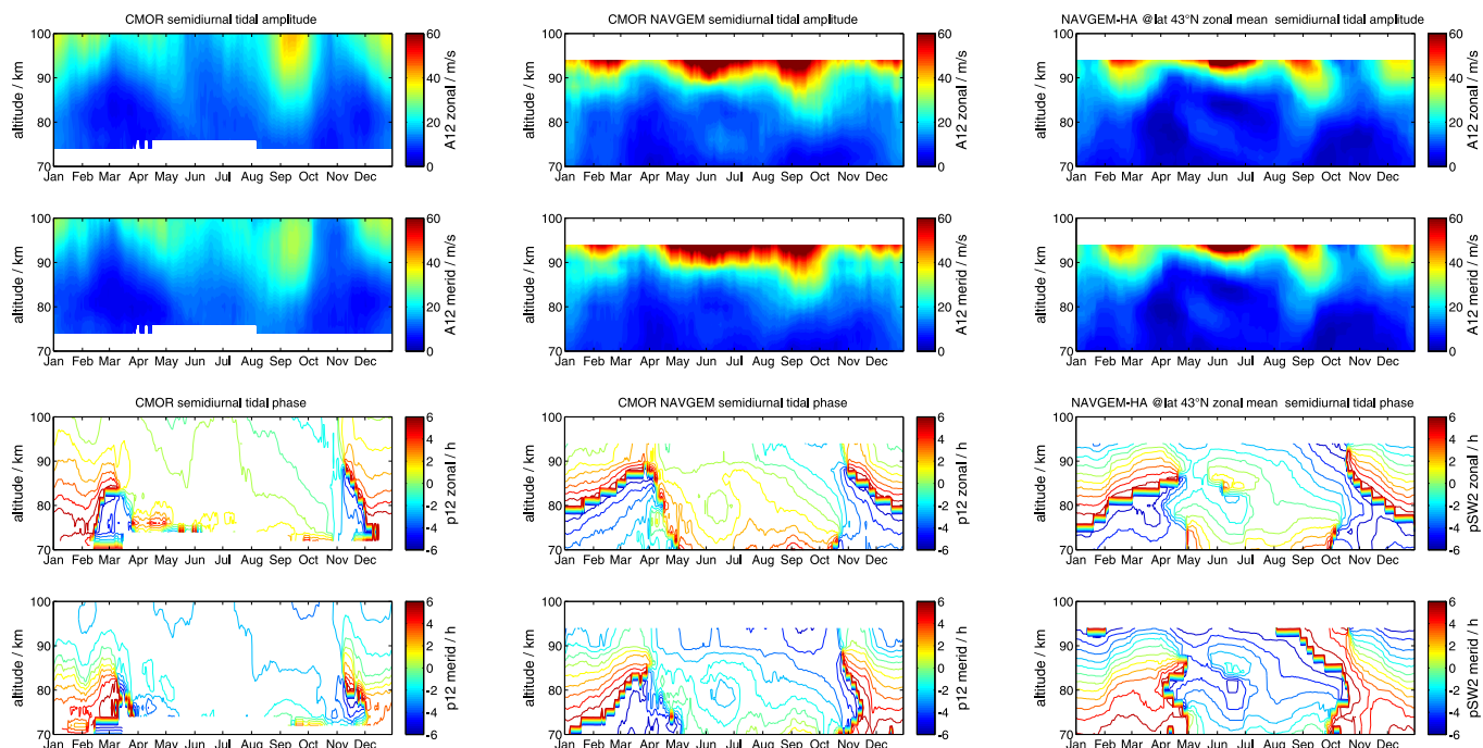
Figure 5. Comparison of semidiurnal seasonal amplitude and phase tidal climatology using a 30-day running median with periodic boundary condition. The left panels show the meteor radar observations above Tavistock ( 43.2^{\circ} N, 80.7^{\circ} W). The central panels show the NAVGEM-HA reanalysis fields for the same period. The right panels visualize the zonal mean tidal amplitude and phase of the SW2.
