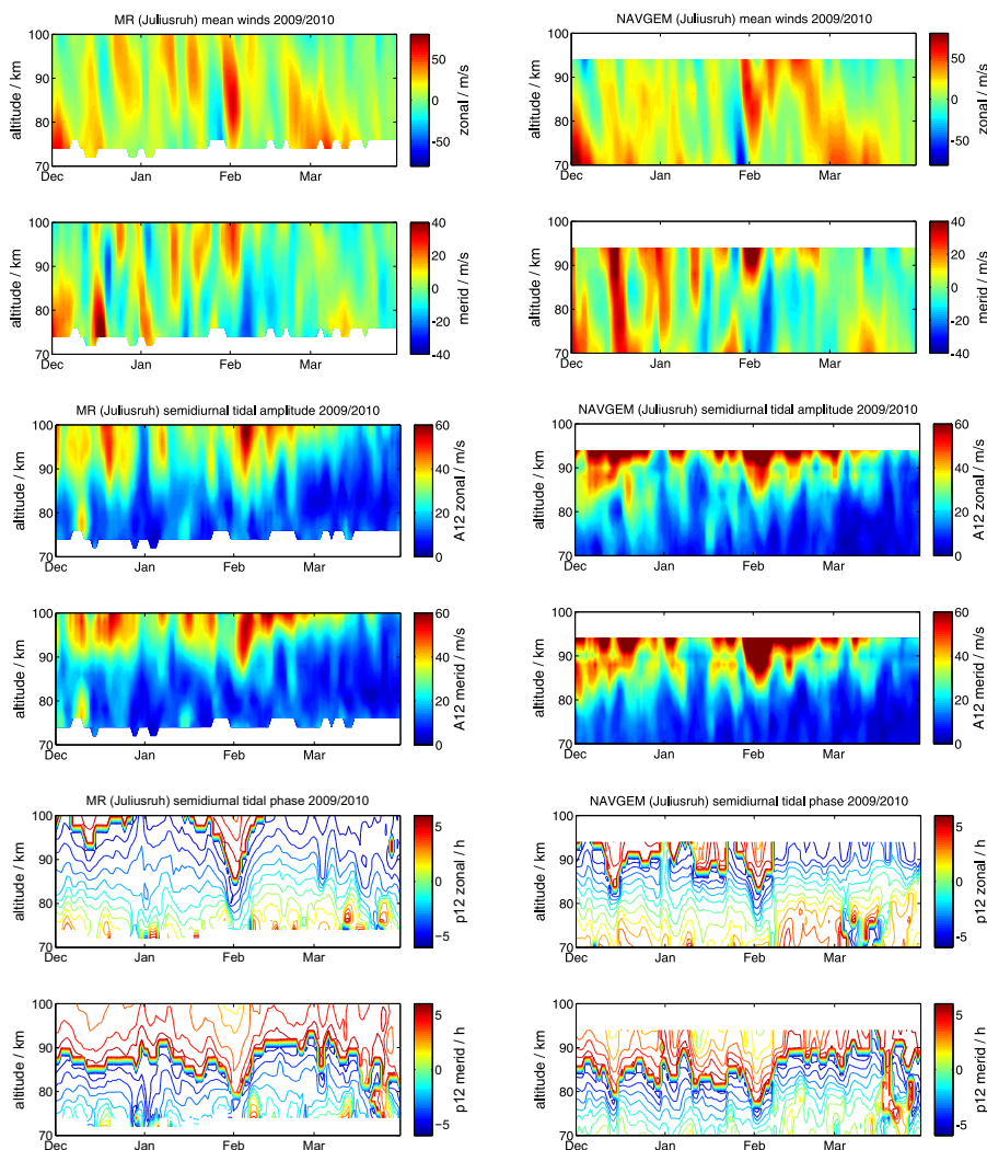
Figure 7. Comparison of meteor radar observations and NAVGEM-HA above Juliusruh during the winter 2009/10 for daily mean zonal and meridional winds (upper two panels), semidiurnal tidal zonal and meridional amplitude (middle panels) and semidiurnal tidal phases (lower two panels).
