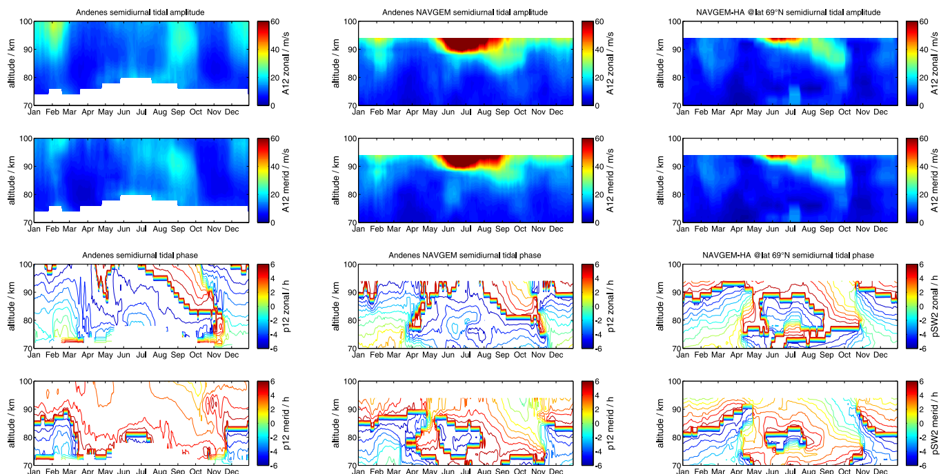
Figure 3. Comparison of semidiurnal seasonal amplitude and phase tidal climatology using a 30-day running median with periodic boundary condition. The left panels show the meteor radar observations above Andenes ( 69^\circ N, 11^\circ E). The central panels show the NAVGEM-HA reanalysis fields for the same period. The right panels visualize the zonal mean tidal amplitude and phase of the SW2.
