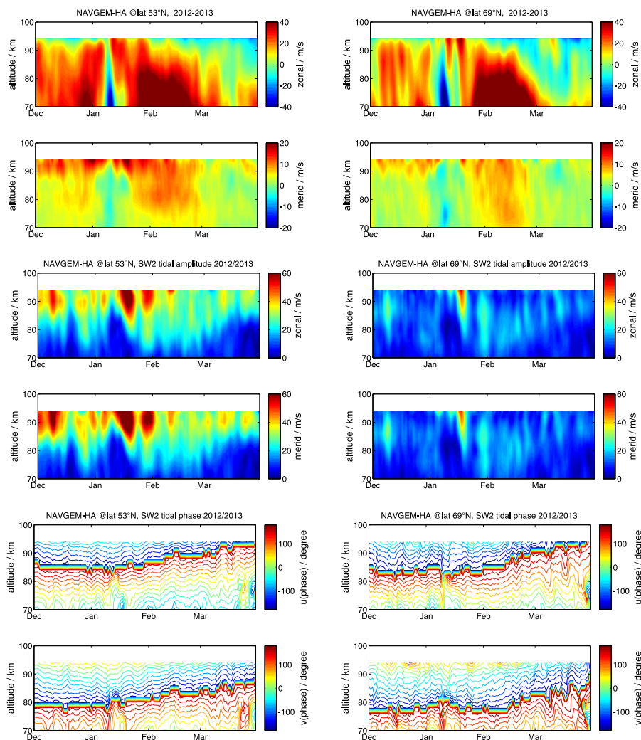
Figure 11. Comparison of global NAVGEM-HA above Juliusruh (left column) and Andenes (right column) during the winter 2012/13 for daily zonal mean zonal and meridional winds (upper two panels), zonal mean semidiurnal tidal zonal and meridional amplitude (middle panels) and zonal mean semidiurnal tidal phases (lower two panels).
