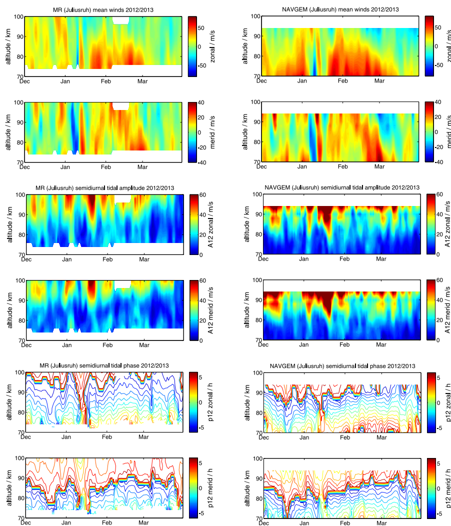
Figure 10. Comparison of meteor radar observations and NAVGEM-HA above Juliusruh during the winter 2012/13 for daily mean zonal and meridional winds (upper two panels), semidiurnal tidal zonal and meridional amplitude (middle panels) and semidiurnal tidal phases (lower two panels).
