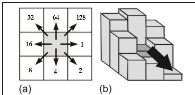
Figure 2 - (a) Coding used to differentiate the eight possible flow directions in the D8 method; (b) assigning the flow direction using the higher slope condition
