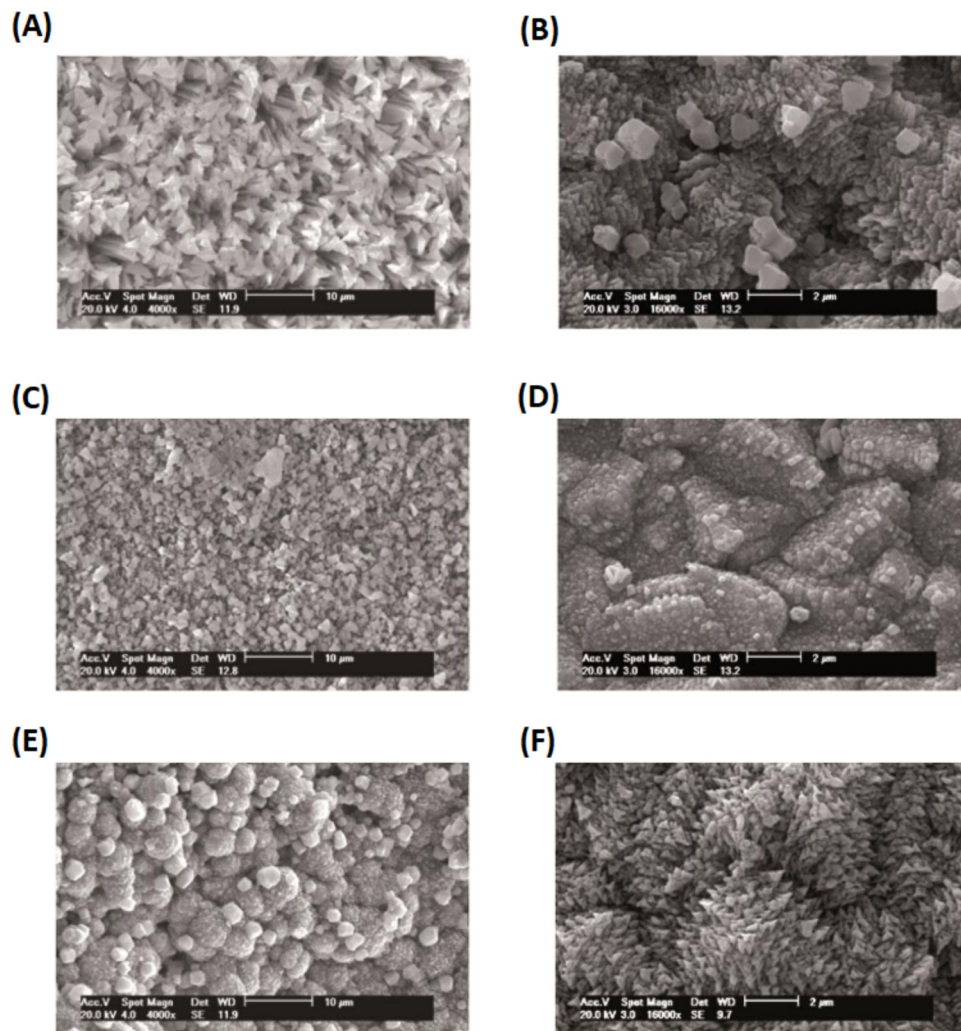
Fig. 6. Degraded layer morphology of the cement-casing interface at different CO 2 -rich brine exposure times: cement after (A) 48 h, (C) 360 h and (E) 720 h; and steel after (B) 48 h, (D) 360 h and (F) 720 h.
