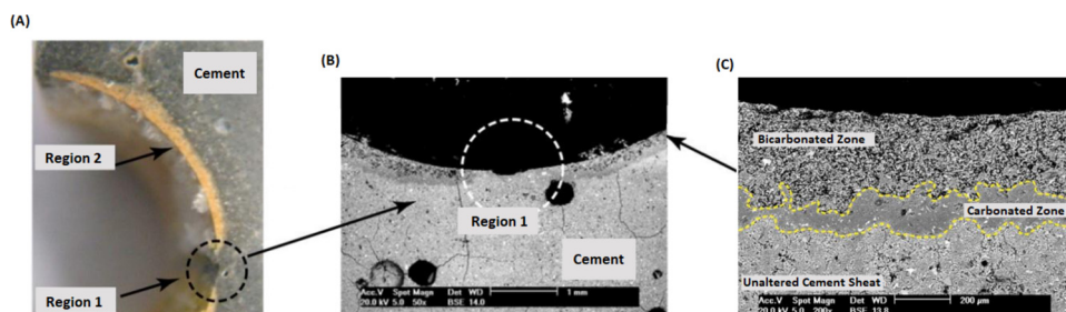
Fig. 4. Cement-casing interfaces of the sample showing interfacial defect: (A) Front view of the cement core, (B) cement-casing interface cross-section SEM image and (C) cement degraded layer cross-section SEM image.
