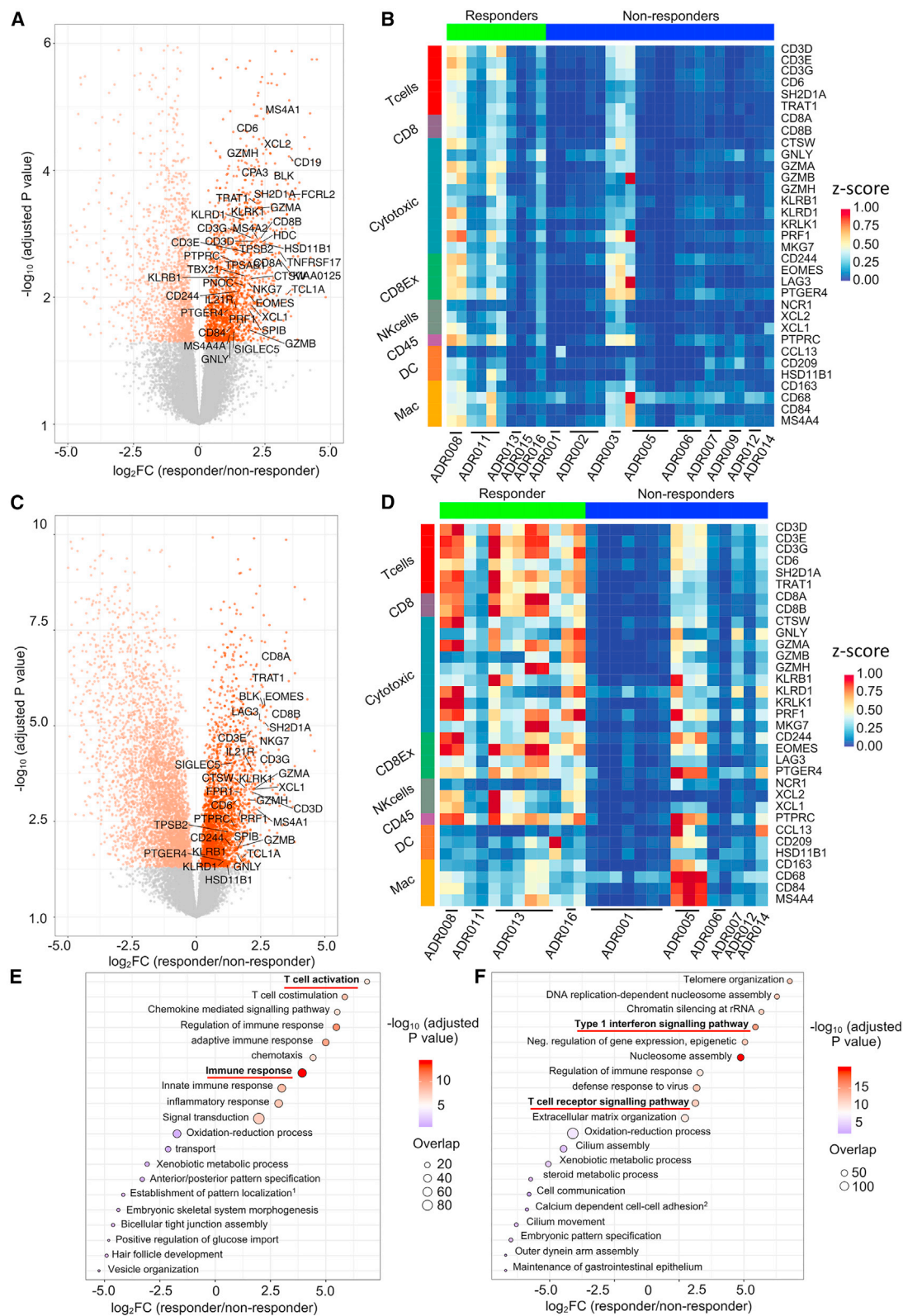
Figure 3. GSEA and immune deconvolution by RNA-seq shows higher levels of immune infiltration and activation in responders compared with non-responders under nivolumab
