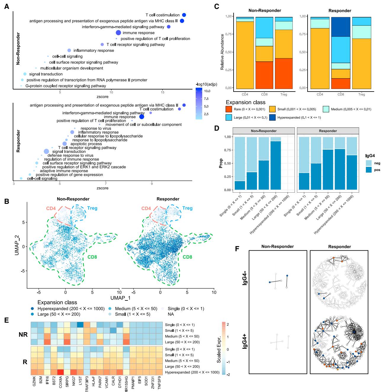
Figure 6. Nivolumab binding correlates with upregulation of T cell activation genes and clones expanded through persistent antigenic stimulation
