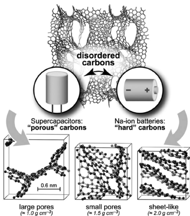
FIG. 16. Machine learning approaches for modeling disordered electrodes. Examples of pore structures in disordered carbons, determined from a combination of machine learning and DFT. 286 Different pore sizes are seen experimentally and are each suited to different applications. Reproduced with permission from Deringer et al. , Chem. Commun. 54 , 5988 (2018). Copyright 2018 The Royal Society of Chemistry and Author(s), licensed under Creative Commons Attribution CC BY 3.0.
